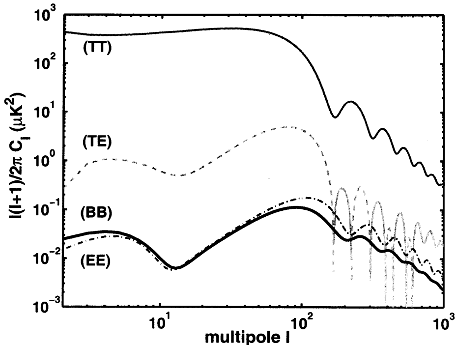
Figure 5.12: The summary of CMB temperature and polarization anisotropies due to relic gravitational waves with n = 1.2 and R = 1 .
