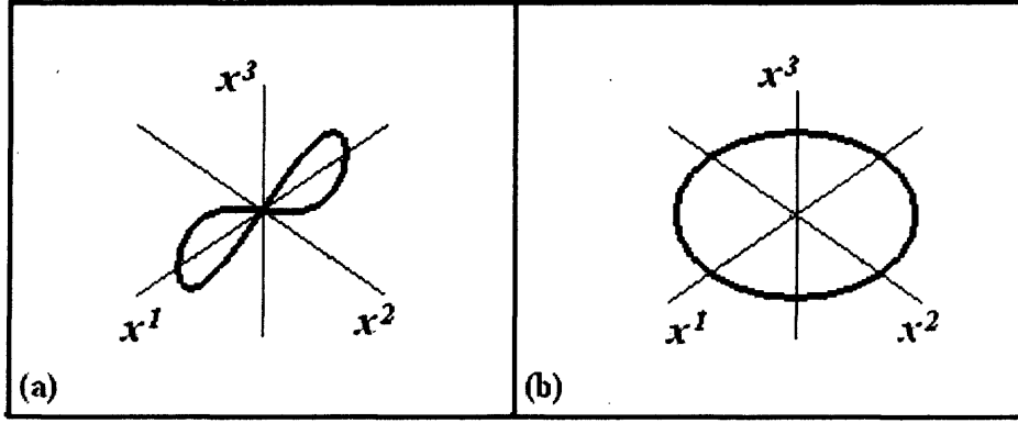
Figure 3.1: The figure a) on the left shows the trajectory of a charged particle in the field of a linearly polarized electromagnetic wave, whereas the figure b) on the right shows the trajectory in the field of a circularly polarized wave.
