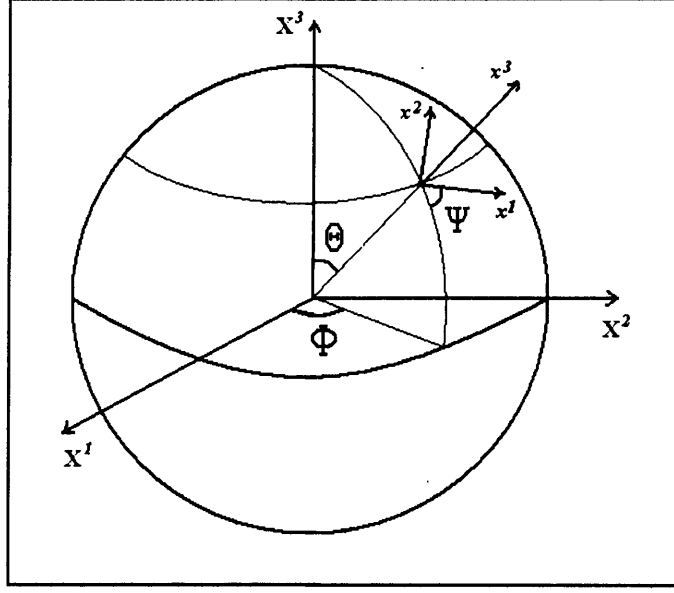
Figure 3.7: The relationship between the coordinate system (x^1, x^2, x^3) adjusted to the wave and the coordinate system (X^1, X^2, X^3) adjusted to the interferometer. The two arms of the interferometer lie along the axes X^1 and X^2 .
