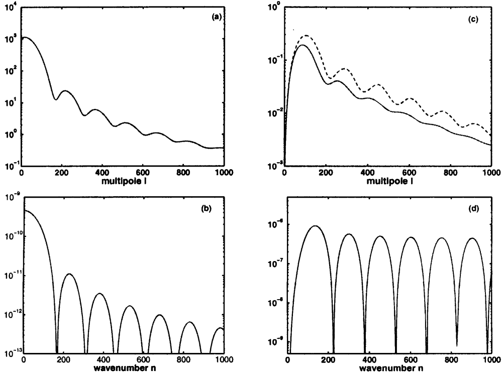
Figure 5.5: The left panel shows (a) the power spectrum of temperature anisotropies \ell(\ell+1)C_\ell^{TT} (in \mu K^2 ) generated by (b) the power spectrum of g.w. metric perturbations (2.14), \beta = -2 . The right panel shows (c) the power spectra of polarization anisotropies \ell(\ell+1)C_\ell^{BB} (solid line) and \ell(\ell+1)C_\ell^{EE} (dashed line), panel (d) shows the power spectrum of the first time derivative of the same g.w. field, Eq. (2.16).
