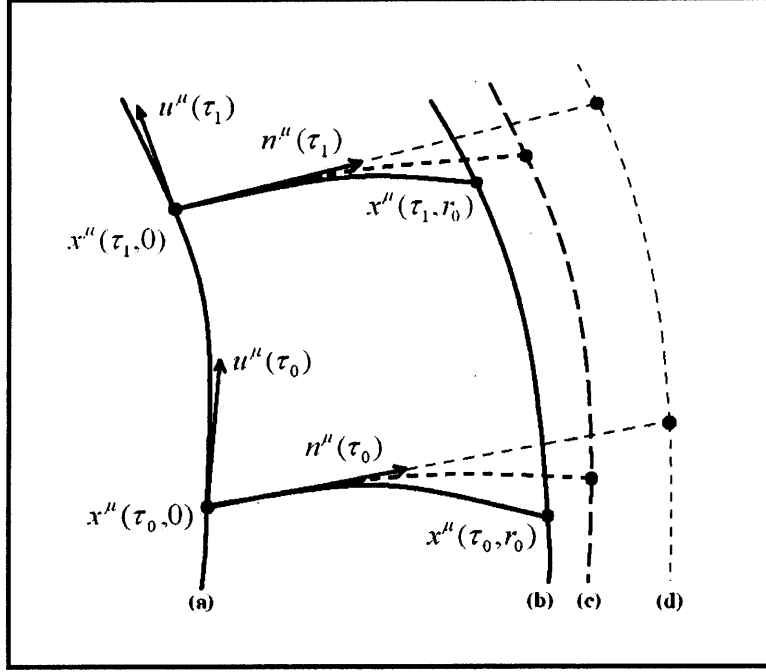
Figure 3.6: Deviation of two nearby geodesics in a gravitational field. Line (a) represents the central geodesic r = 0 and line (b) represents the nearby geodesic r = r_0 . u^\mu is the unit tangent vector to the central world line, n^\mu is the tangent vector to the curve \tau = \text{const} . The lines (d) and (c) are the corresponding first and second order approximations to the exact nearby geodesic (b).
