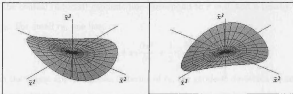
Figure 3.5: The figure shows the deformations of a circular disk of free test particles under the action of a linearly polarized g.w. ( h_+ \neq 0, h_\times = 0 ). The “magnetic” contribution is responsible for the displacements along the \bar{x}^3 axis. The two pictures show the configurations at the moments of time separated by a half of period.
