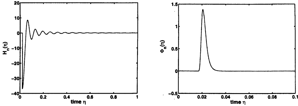
Figure 5.2: The ‘source’ functions H_{n,s}(\eta) and \Phi_{n,s}(\eta) ( n = 100 ) of temperature and polarization anisotropies (the normalization is chosen such that h_n(\eta_r) = 1 ).
