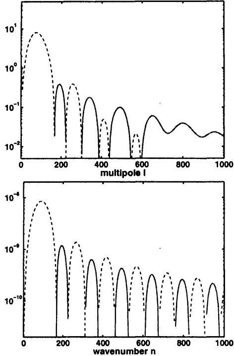
Figure 5.6: The bottom panel shows the spectrum (5.50) of gravitational waves, whereas the top panel shows the angular power spectrum \ell(\ell + 1)C_\ell^{TE} caused by these waves. The negative values of these functions are depicted by broken lines.
