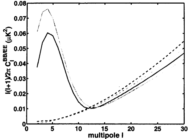
Figure 5.9: The reionization ‘bump’ in the polarization power spectra. The dashed lines show the spectra when the reionization era is ignored. The solid lines include both eras. The darker lines are for B -mode, and the lighter lines for E -mode.
