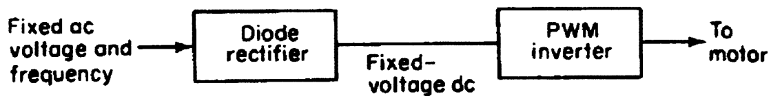
Figure 3.4 PWM inverter dc link converter supply [3.1]
