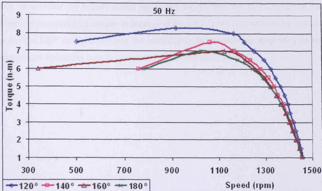
Figure 9.5 Speed torque curves of the motors with coil pitches 120^\circ , 140^\circ , 160^\circ , 180^\circ at different torques under PWM supply voltage at 50 Hz modulation frequency and 4 kHz switching frequency
