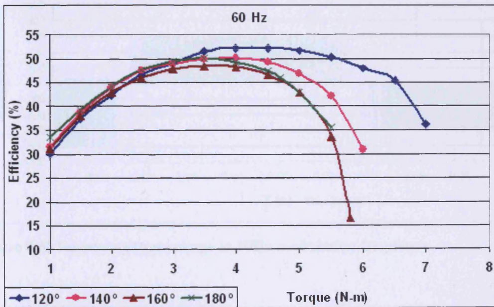
Figure 8.44 Efficiencies of the motors with coil pitches 120°, 140°, 160°, 180° at different torques under PWM supply voltage at 60 Hz modulation frequency and 4 kHz switching frequency
