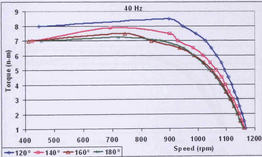
Figure 9.4 Speed torque curves of the motors with coil pitches 120°, 140°, 160°, 180° at different torques under PWM supply voltage at 40 Hz modulation frequency and 4 kHz switching frequency
