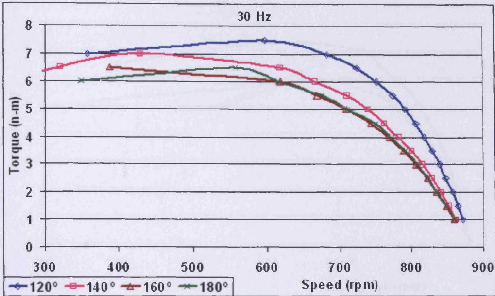
Figure 9.3 Speed torque curves of the motors with coil pitches 120°, 140°, 160°, 180° at different torques under PWM supply voltage at 30 Hz modulation frequency and 4 kHz switching frequency
