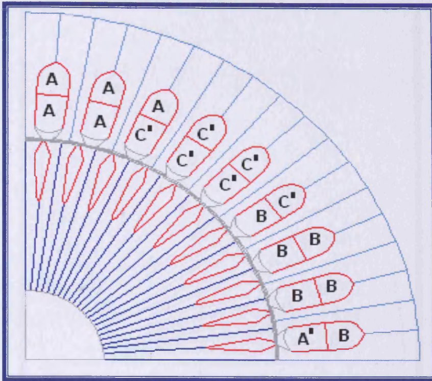
Figure 7.6 Stator winding layout of the 160° coil pitch motor
