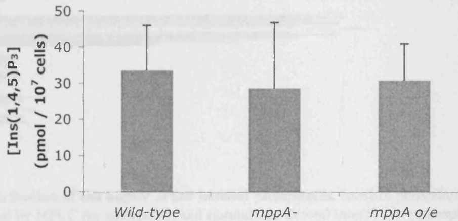
Figure 3.8: Analysis of inositol phosphate abundance in mppA mutants. Cells extracts were prepared and analysed by (A) HPLC-MDD, and (B) the Ins(1,4,5)P 3 – specific isotope dilution assay. Isomers separated by HPLC were identified as: a – unresolved InsP 3 isomers; b – Ins(1,2,3,5)/(1,2,4,6)P 4 ; c – Ins(1,2,4,5)P 4 ; d – Ins(1,2,5,6)P 4 ; e – Ins(1,4,5,6)P 4 ; f – Ins(1,2,3,4,6)P 5 ; g – Ins(1,2,3,4,5)P 5 ; h – Ins(1,2,4,5,6)P 5 ; i – Ins(1,3,4,6)/(1,2,3,4)P 4 ; j – Ins(2,4,5,6)P 4 ; k – Ins(1,3,4,5,6)P 5 .
