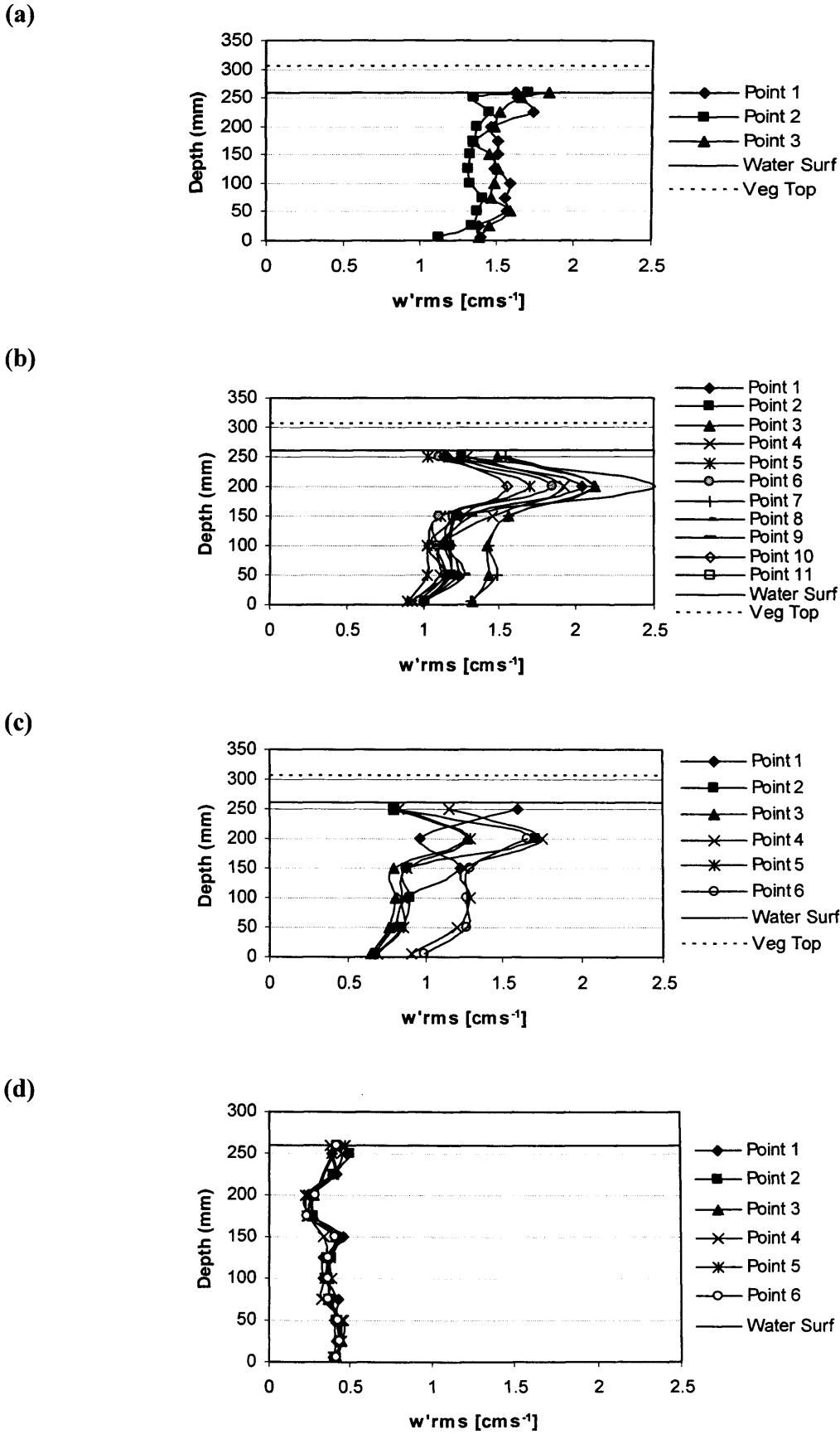
Fig. 5.21 Time-averaged rms velocity fluctuations ( w'rms ) [cms -1 ] for four configurations: (a) high, (b) medium, (c) low, and (d) no vegetation.
