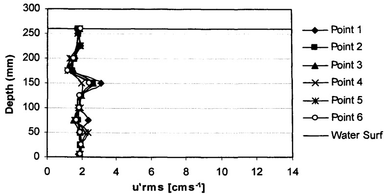
Fig. 5.19 Time-averaged rms velocity fluctuations ( u'_{rms} ) [cms -1 ] for four configurations: (a) high, (b) medium, (c) low, and (d) no vegetation.
