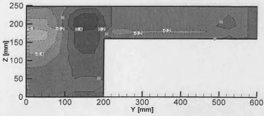
Fig. 4.5 Time-averaged vertical velocity ( \bar{W} ) [ \text{cm s}^{-1} ] at cross-section 4.4 and for four configurations: (a) high, (b) medium, (c) low, and (d) no vegetation.
