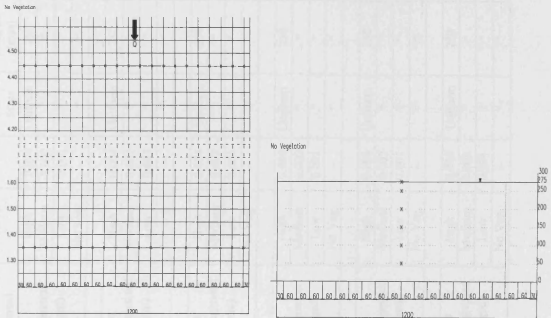
Fig. 3.14 Layout and details of the partial half two-sided submerged and emergent vegetation experiments in the wide channel showing the measuring point locations and two vertical velocity profiles 4.4 and 1.4 for four configurations: (a) high, (b) medium, (c) low, and (d) no vegetation.
