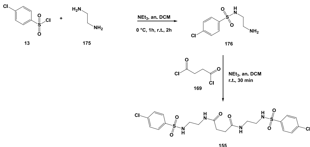
Scheme 3.5: Synthetic pathway for compound 155
