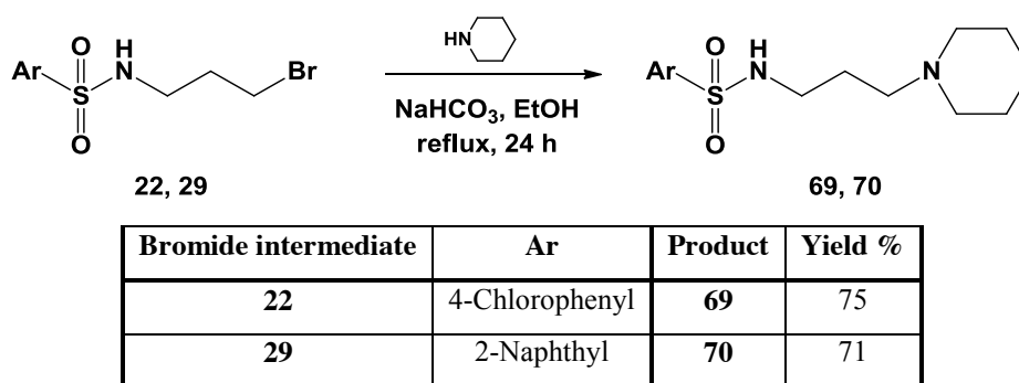
Scheme 2.4: Synthesis of compounds 69 and 70
