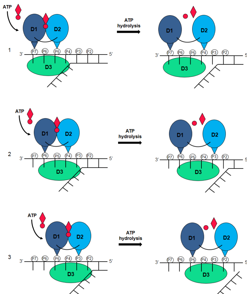
Figure 1.14: Representation of NS3 movements along a RNA tracking strand 102
