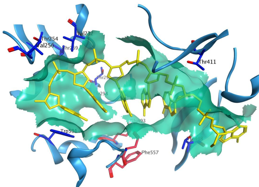
Figure 4.1: Residues with low RMSD values (<3 Å in blue, < 2Å in pink) shown within the 3KQH RNA binding cleft
