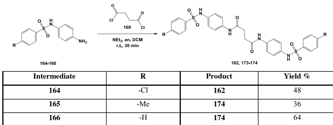
Scheme 3.4: Final step for the synthesis of compounds 162 , 173-174
