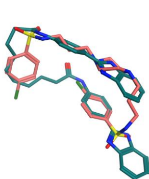
Figure 3.8: Aligned compounds 12 and 5e
