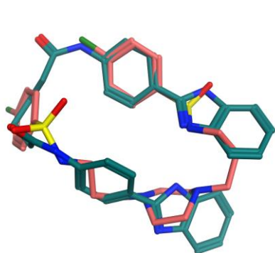
Figure 3.6: Aligned compounds 12 and 5b
