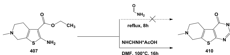
Scheme 4.33: Attempts for the synthesis of compound 410
