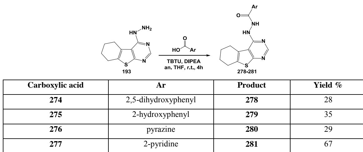
Scheme 4.9: Synthesis of hydrazide compounds 278-281
