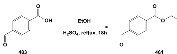
Scheme 5.2: Synthesis of starting bendaldehyde 461
