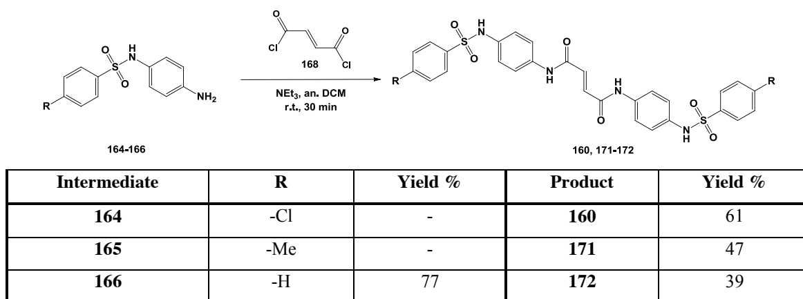
Scheme 3.3: Final step for the synthesis of compounds 160 , 171-172
