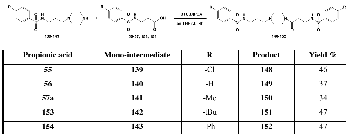
Scheme 2.19: Pathway for the synthesis of compounds 148-152
