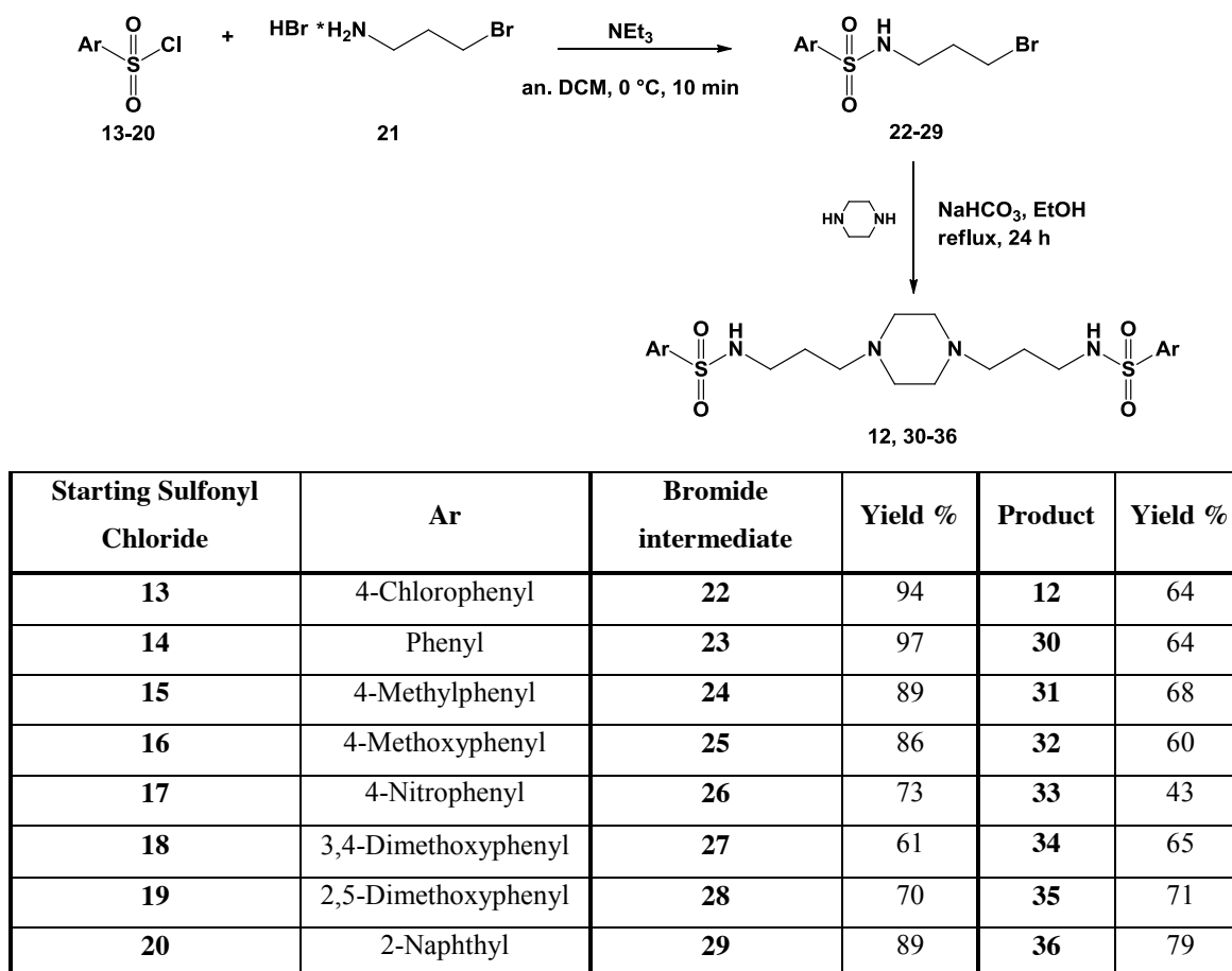
Scheme 2.1: Pathway for the synthesis of compounds 12 , 30-36
