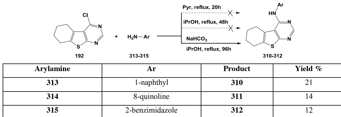
Scheme 4.7: Synthesis of compounds 310-312
