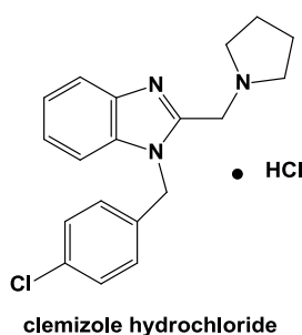
Figure 1.8: Chemical structure of clemizole hydrochloride
