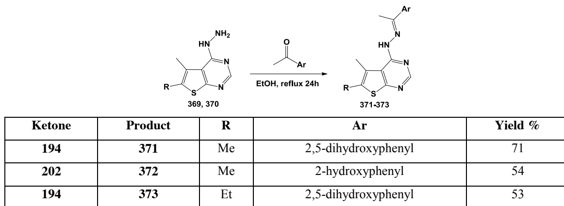
Scheme 4.19: Synthesis of compounds 371-373
