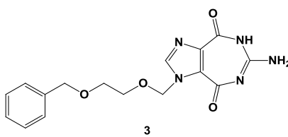
Figure 1.17: Chemical structure of compound 3
