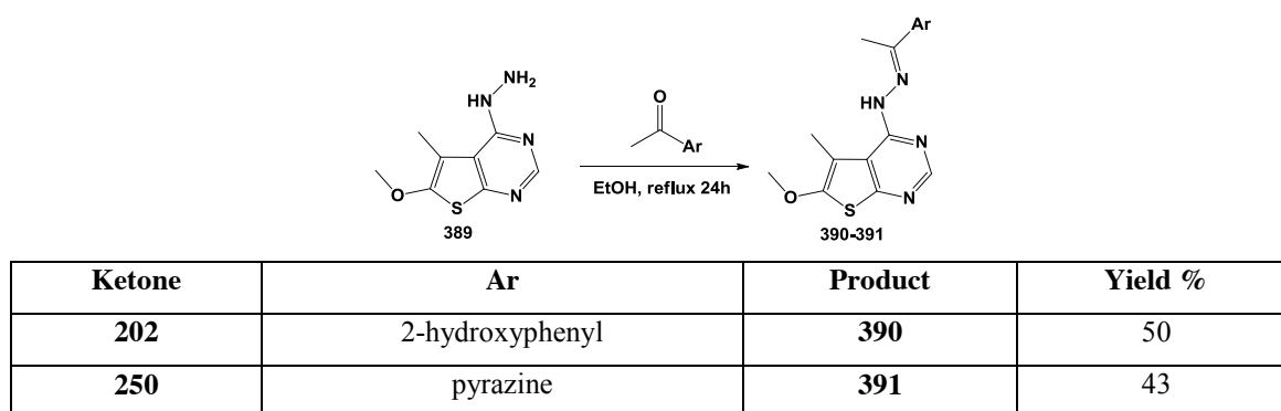
Scheme 4.25: Synthesis of compounds 390-391
