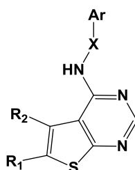
187: R_1, R_2 = C_4H_8 , X = NCCH_3 , Ar = 2,5-OH-Ph
