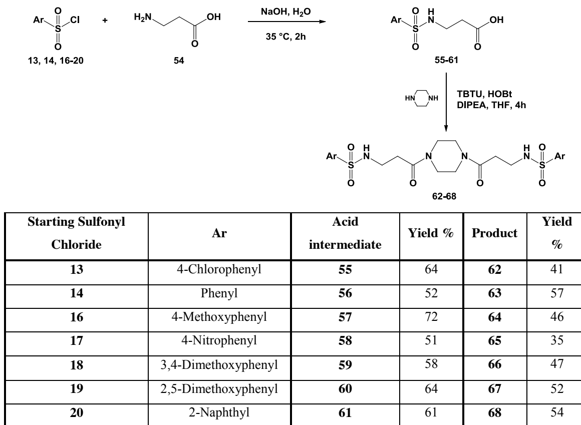
Scheme 2.3: Pathway for the synthesis of compounds 62-68
