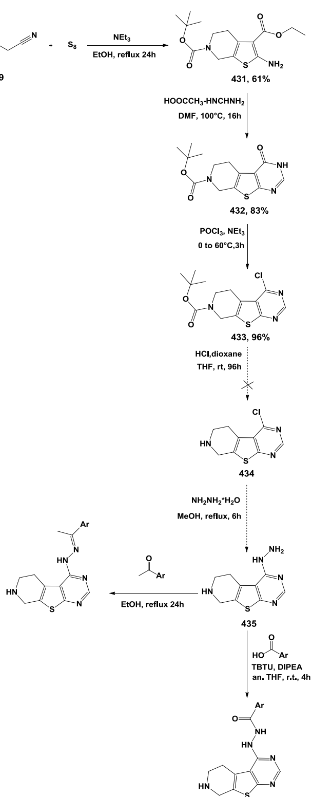
Scheme 4.34: First synthetic strategy attempted for tetrahydropyridine compounds
