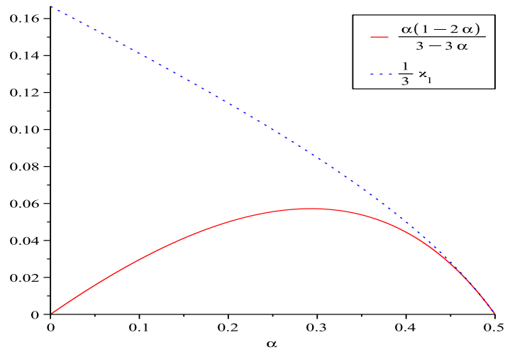
Figure 1: Graphs of \varkappa_1/3 and \frac{\alpha(1-2\alpha)}{3(1-\alpha)} for d = 1 .
