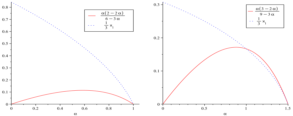
Figure 2: Graphs of \varkappa_1/3 and \frac{\alpha(d-2\alpha)}{3(d-\alpha)} for d = 2 and 3 .
