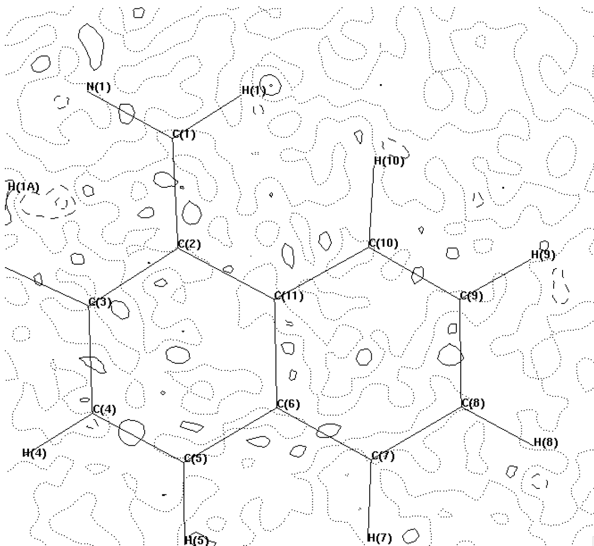
Figure 2 Residual density from multipole model in the plane of C(1), N(1) and C(2), displayed at the 0.1 \text{ e.}\text{\AA}^{-3} contour level.
