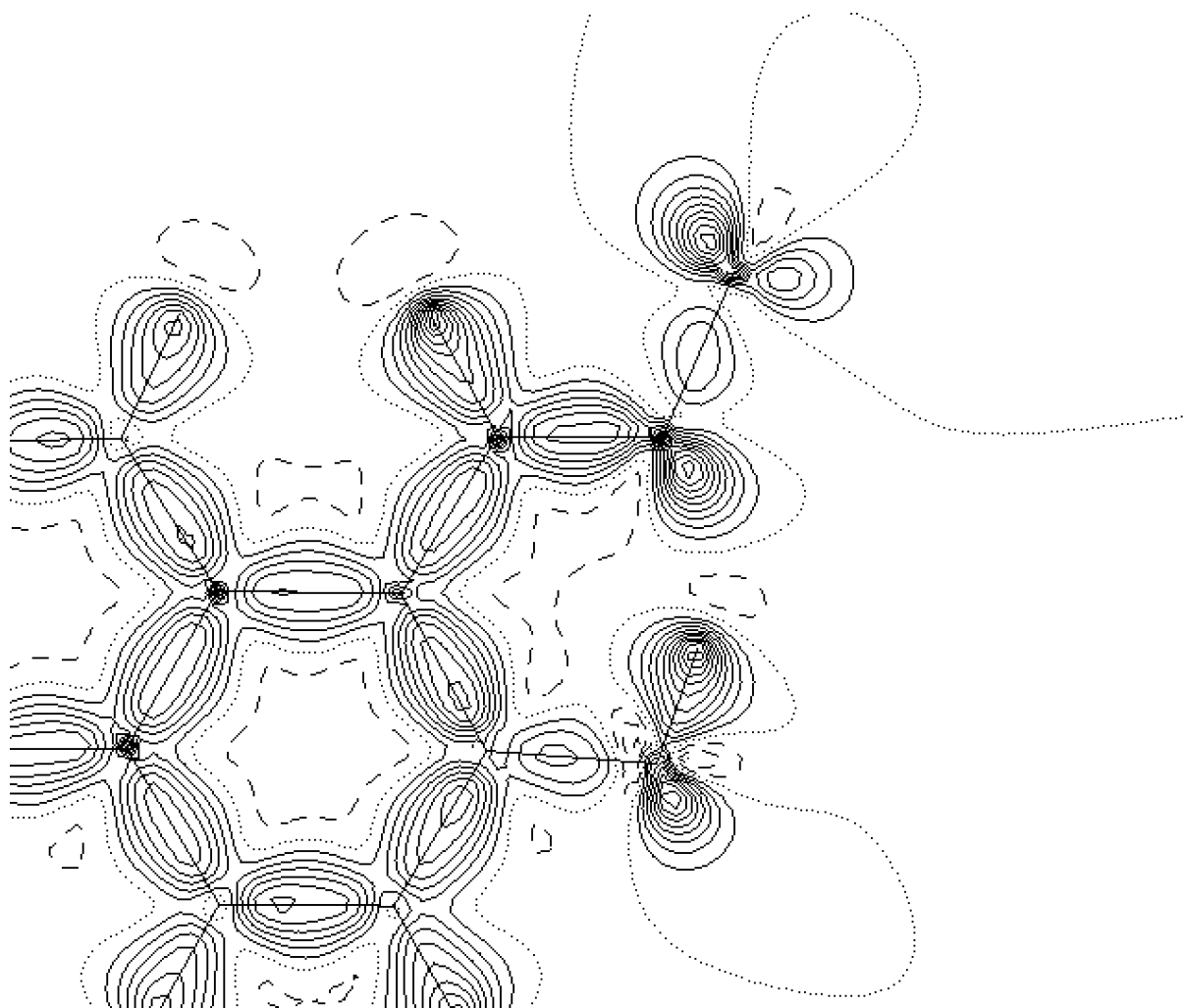
Figure 3: Static deformation density in plane of C(1), N(1) and C(2), plotted with contours at regular the 0.1 e.Å -3 intervals.
