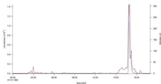
Figure 6. Radio-HPLC was performed in order to confirm the formation of 25 . The fluoridation product was co-eluted with reference compound 24 after 17.2 min (MeCN/H 2 O 10:1, flow rate 1 mL min -1 ). The profile of the radio-HPLC diagram is consistent with the radio-TLC diagram shown above.
