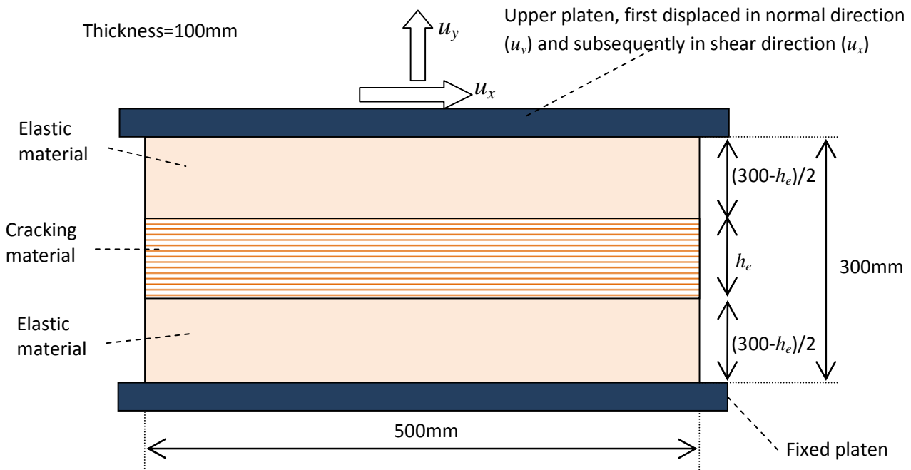
Figure 12. Idealised arrangement considered in Example 1
