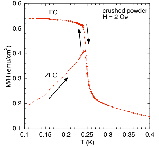
FIG. 4: M/H vs T for the crushed powder for H = 2 Oe measured in a ZFC-FC procedure.
