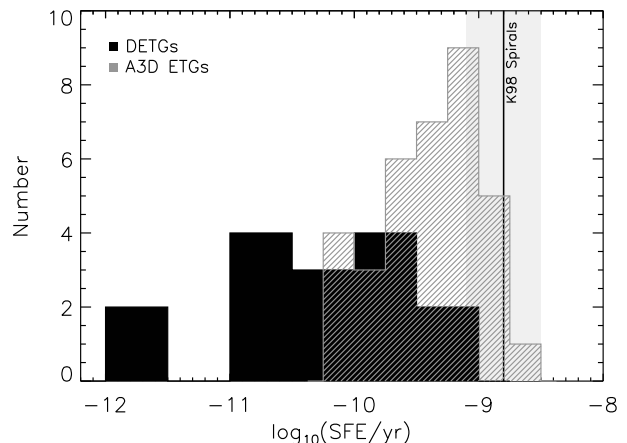
Figure 5. Histogram of the star formation efficiency (SFE=SFR/ M_{\text{H}_2} ) in our DETGs (black histogram) and ATLAS 3D ETGs (grey shaded histogram). The average SFE of the spiral galaxies from Kennicutt (1998) is also shown as a black vertical line, with a grey bar showing the standard deviation of their SFEs around the mean.
