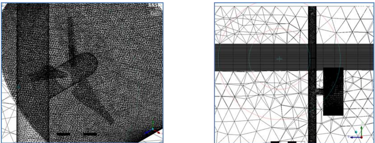
Figure 3. Meshing arrangement for the VOF.
