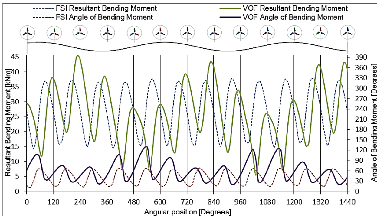
Figure 9. Transient bending moment for the VOF and FSI model.
