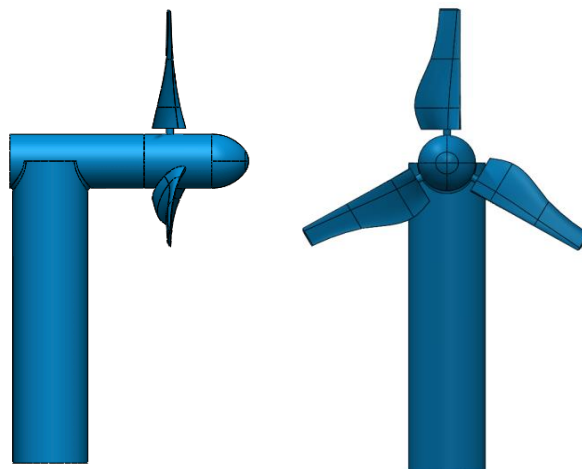
Figure 2. Side and front view of turbine-stanchion arrangement for all the models.
