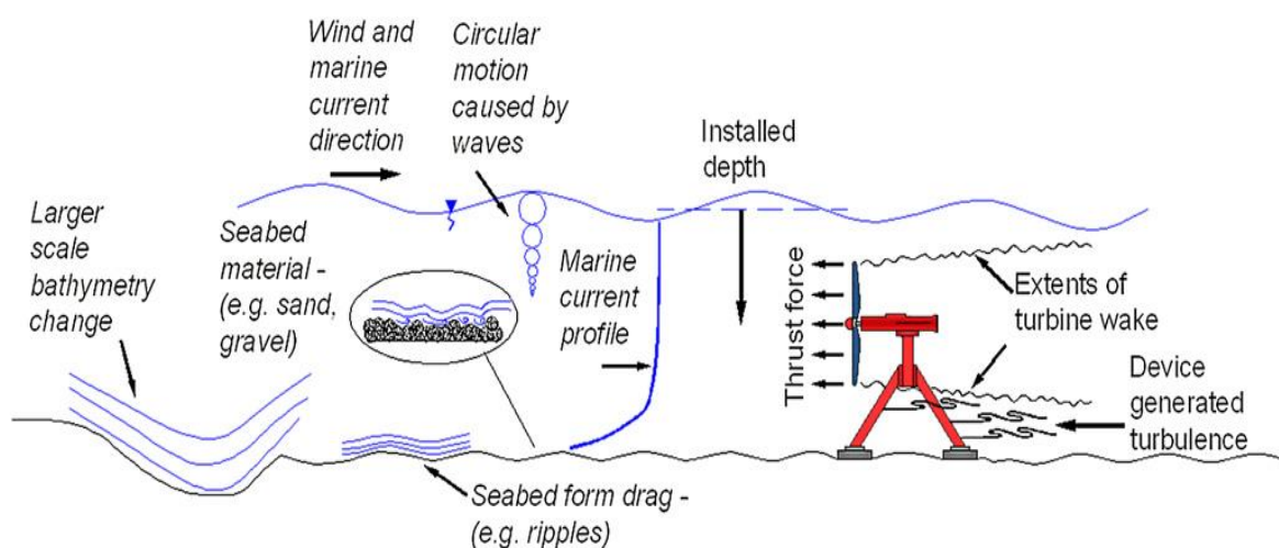
Figure 1 Variables affecting the flow field around tidal turbines [12].
