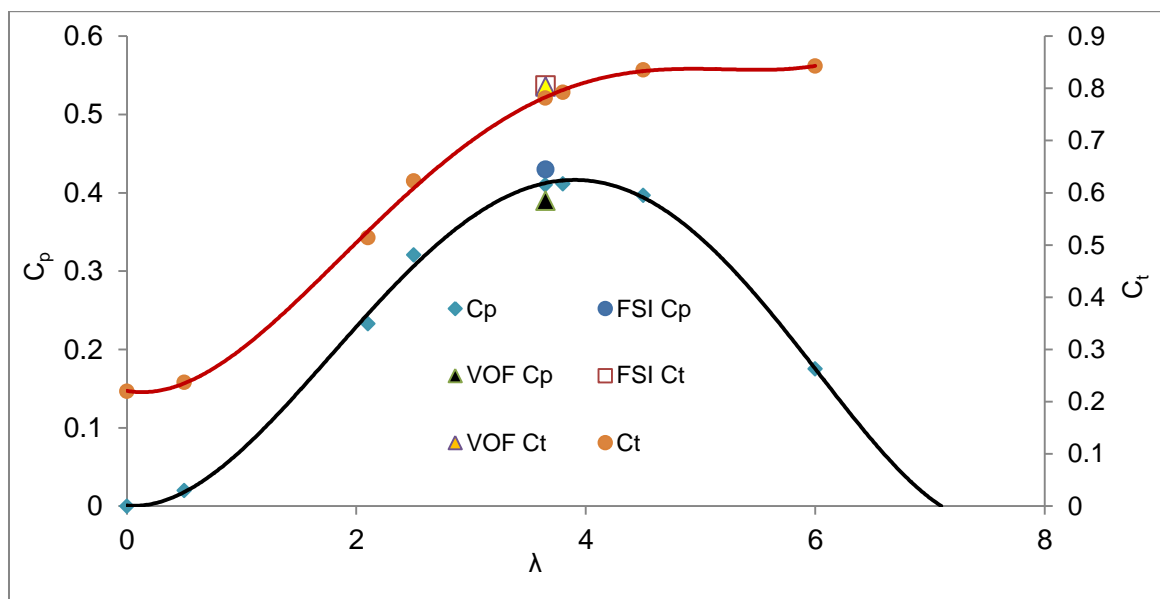
Figure 6. Turbine performance characteristics (uncoupled CFD) with peak power and thrust values for the VOF and FSI models.
