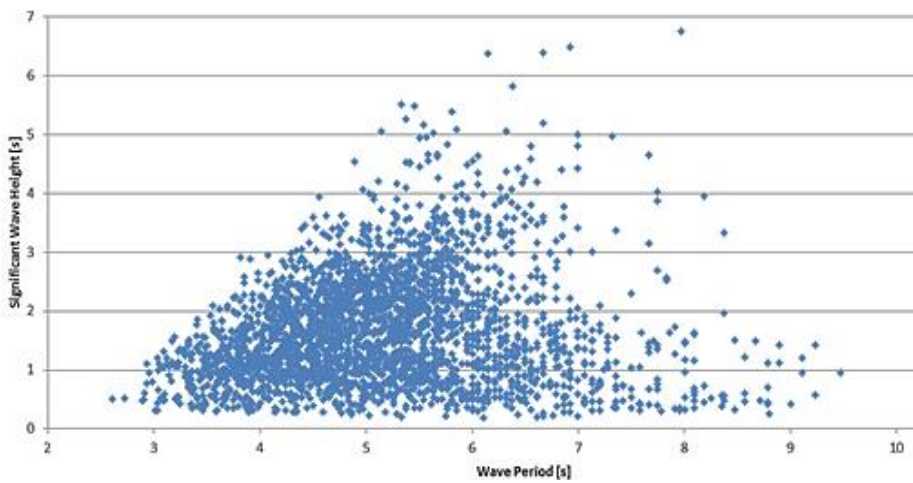
Figure 4. Scatter plot of waves at Gower based on their significant periods and wave heights [19].
