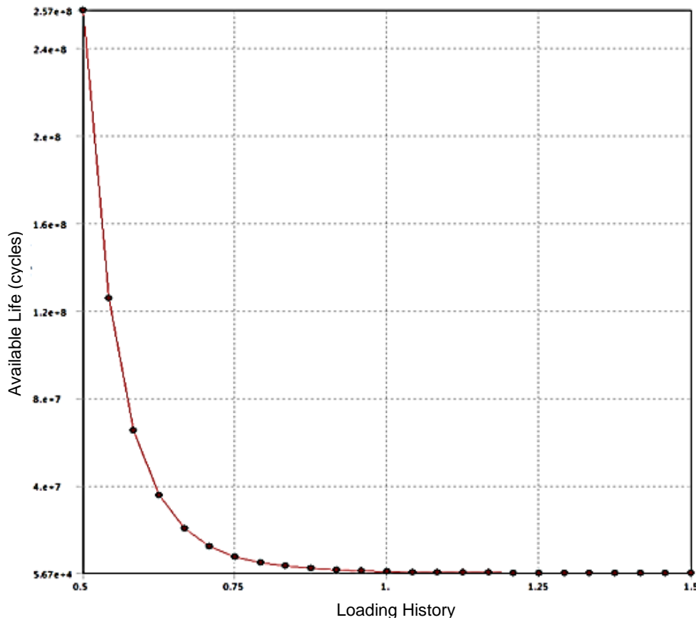
Figure 11. Life prediction curve.
