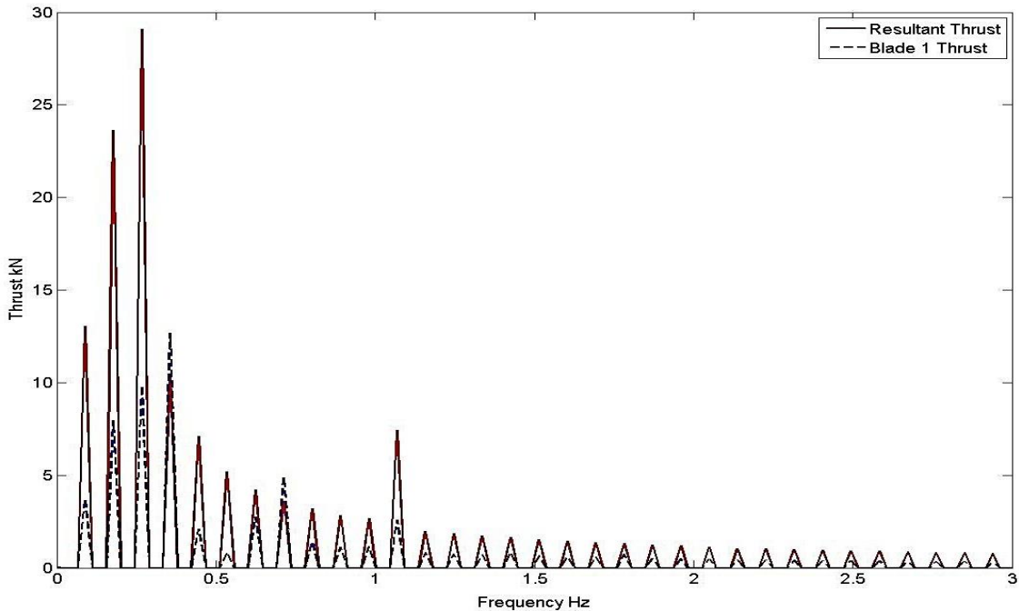
Figure 13 : Frequency spectrum for the axial thrust loading on the turbine for the VOF model showing frequency spectrum associated with a single blade (blue) and the resultant (red) .
