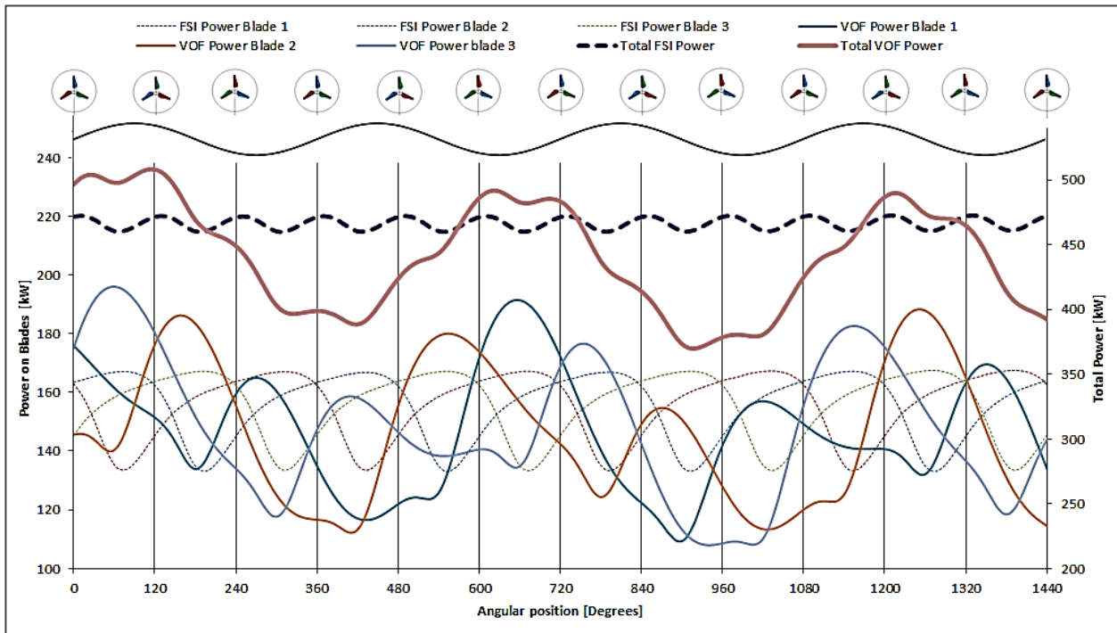
Figure 8. Transient power curves for the VOF and FSI models.
