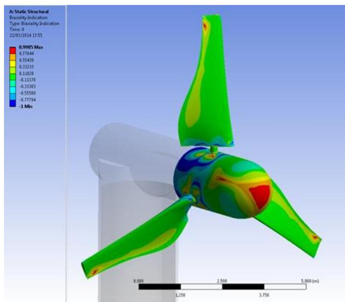
Figure 10. Biaxial Indication.
