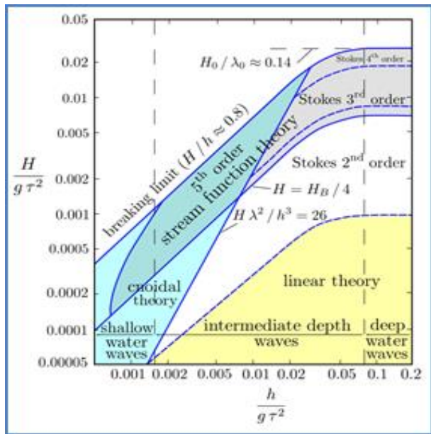
Figure 5. Non dimensionalised water depth and wave height to determine wave regime [20].
