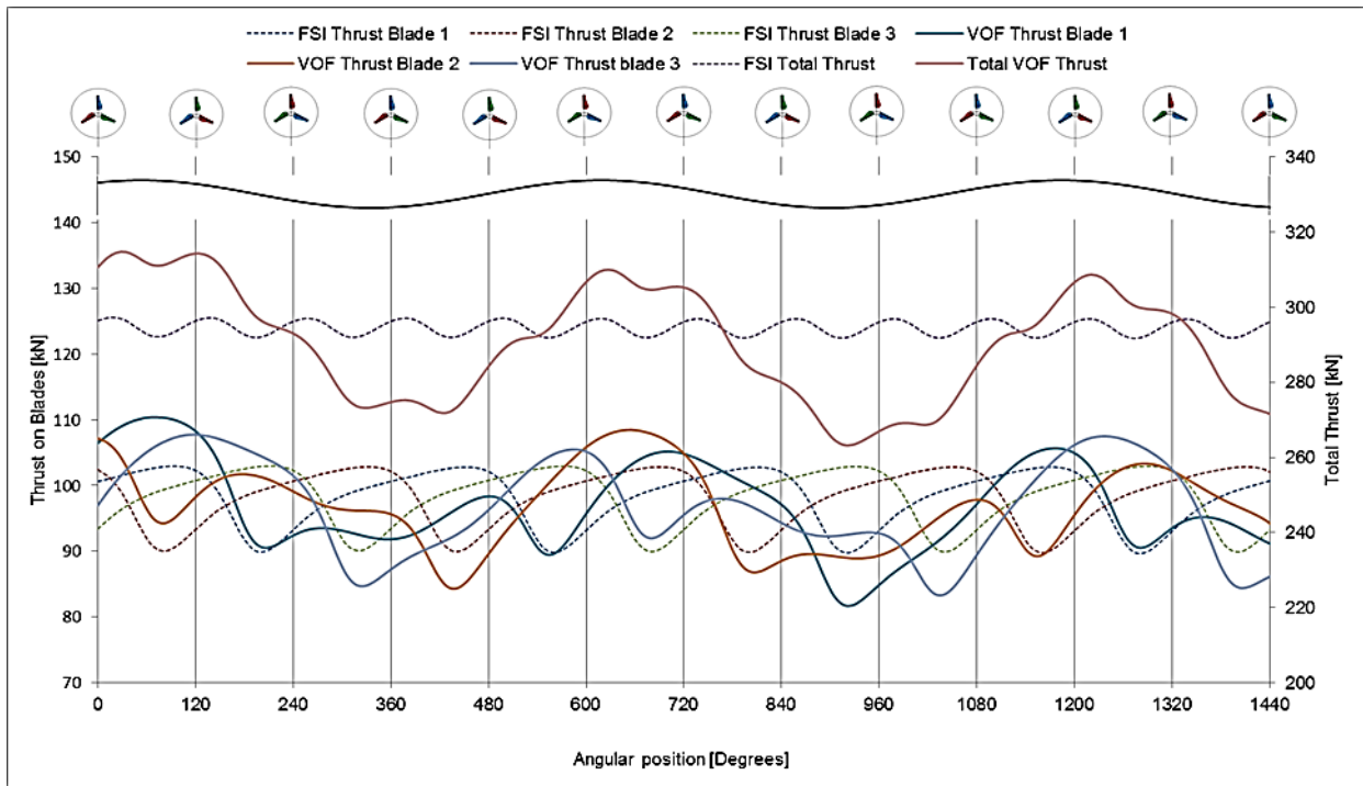
Figure 7. Transient thrust curves for the VOF and FSI models.
