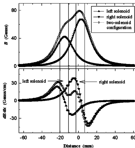
FIG. 2. Magnetic field strength and field gradient generated by two solenoids with different numbers of turns along a common central axis (left solenoid: solenoid radius R=14 mm, current i=1 A, number of turns N=100 , and solenoid length L=10 mm; right solenoid: R=14 mm, i=1 A, N=160 , and L=10 mm. The distance between the centers of the two solenoids is 18.3 mm).
