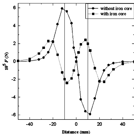
FIG. 1. Magnetic force at the center of a 15 mm ferrofluid plug along the central axis of a solenoid with or without an iron core. The center of the solenoid is at x=0 . The solenoid parameters are length L=20 mm, radius R=14 mm, and number of turns N=100 ; the current i=1 A and the thickness t of the core =2 mm.
