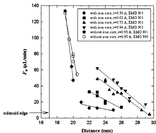
FIG. 3. Average flow rate at different currents as a function of the distance between the center of a ferrofluid plug and of a 17 mm long solenoid with 80 turns. The radius of the flow channel is 0.5 mm, the radius of the solenoid is 6.25 mm, and the thickness of the iron core is 2 mm. The ferrofluid was diluted with toluene at a weight ratio of 1:1.
