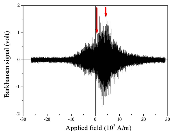
FIG. 4. Simulated BE signal for the hardened steel sample with a nominal case depth of 0.36 mm.
