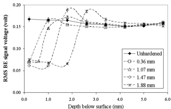
FIG. 2. Variation of the rms BE signal voltage with depth for the unhardened and surface-hardened samples with different case depths.
