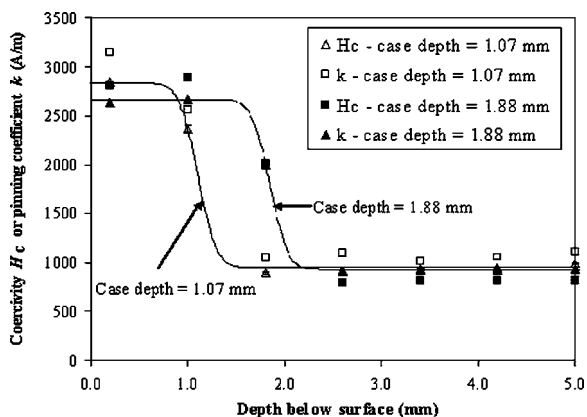
FIG. 3. Coercivity and pinning coefficient k vs depth for the surface-hardened samples with nominal case depths of 1.07 mm and 1.88 mm.
