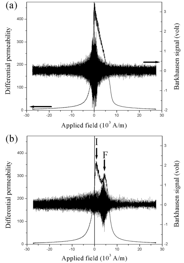
FIG. 1. Plots of the differential permeability and BE signal as a function of applied field for the (a) unhardened sample, and (b) surface hardened sample with a nominal case depth of 0.36 mm.
