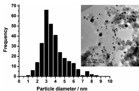
Figure 1. Particle size histogram from the TEM analysis and a representative image.
