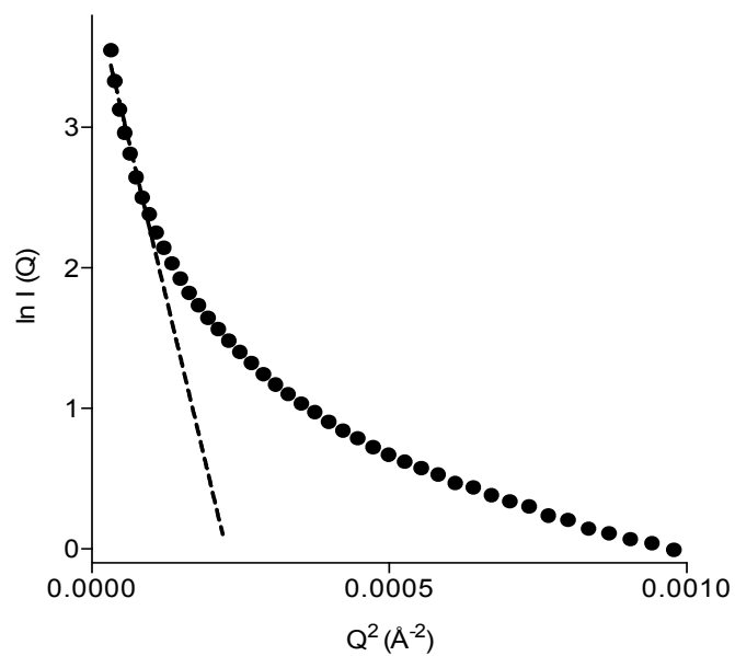
Figure S1. Example of a Guinier plot of SANS data, used to calculate R_g . Graph shows data for LPS (10 mg/mL in D_2O ).
