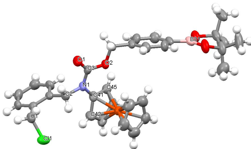
Figure 1. Molecular structure of compound 11 as determined by X-ray crystallography.
