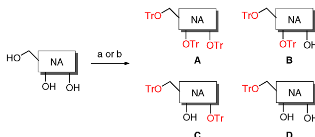
Scheme 1. General synthetic methods to trityl compounds 5-24 A-D . Reagents and conditions: a) trityl chloride (2.8 equiv), pyridine ( 4.5 \text{ mL mmol}^{-1} ), 80^{\circ}C , 18 h; b) trityl chloride, (2.8 equiv), DMAP (2.8 equiv), pyridine ( 4.5 \text{ mL mmol}^{-1} ), 80^{\circ}C , 18 h.
