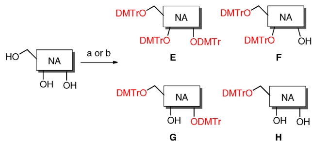
Scheme 2. General synthetic method to 4,4'-dimethoxytrityl compounds 5–20E–H. Reagents and conditions: a) 4,4'-dimethoxytrityl chloride, (2.8 equiv), pyridine (4.5 mL mmol -1 ), 80 °C, 18 h; b) 4,4'-dimethoxytrityl chloride, (2.8 equiv), DMAP (2.8 equiv), pyridine (4.5 mL mmol -1 ), 80 °C, 18 h.
