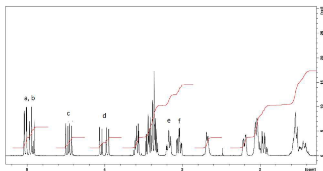
Figure 1 Section of the ^1\text{H} NMR spectrum of \text{chxnPS}_2 . The peaks labelled a-d are those of the benzylic hydrogens \alpha to the nitrogens and those labelled e,f are the methine hydrogens.
