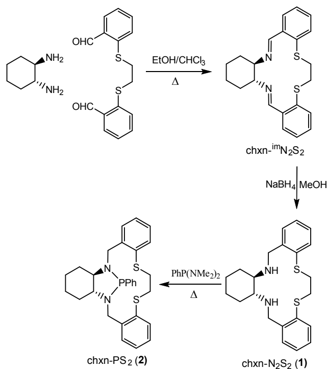
Scheme 1 Synthesis of \text{chxn-N}_2\text{S}_2 and \text{chxnPS}_2
