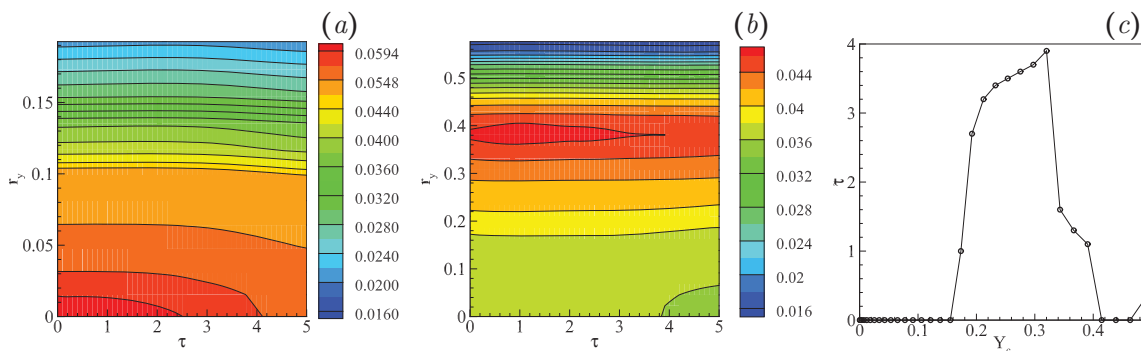
Figure 6. Section of the space (r_\pi, r_y, \tau, Y_c) in the (a) (r_\pi = 2.4, Y_c = 0.1) -plane and (b) (r_{pi} = 2.4, Y_c = 0.3) -plane colored with \langle \delta\theta^2 \rangle for Ra = 1.7 \times 10^5 . (c) Characteristic time scale \tilde{\tau}(Y_c) as a function of Y_c for Ra = 1.7 \times 10^5 .
