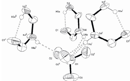
Figure 10: View of the hydrogen bonding interactions of 6 .
