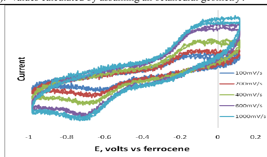
Figure 2: Cyclic voltammetry for 4 vs \text{Fc}/\text{Fc}^+ . (Pt working electrode; 0.1 M TBAH; conc of 4 < 0.1 mM)
