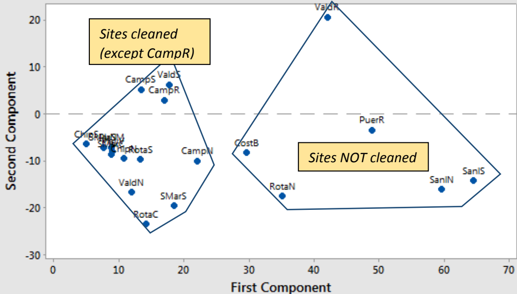
Score Plot of CL04, ..., YYXX Cadiz: 20 sites; 59 categs. (Covariance, non-stand.)
