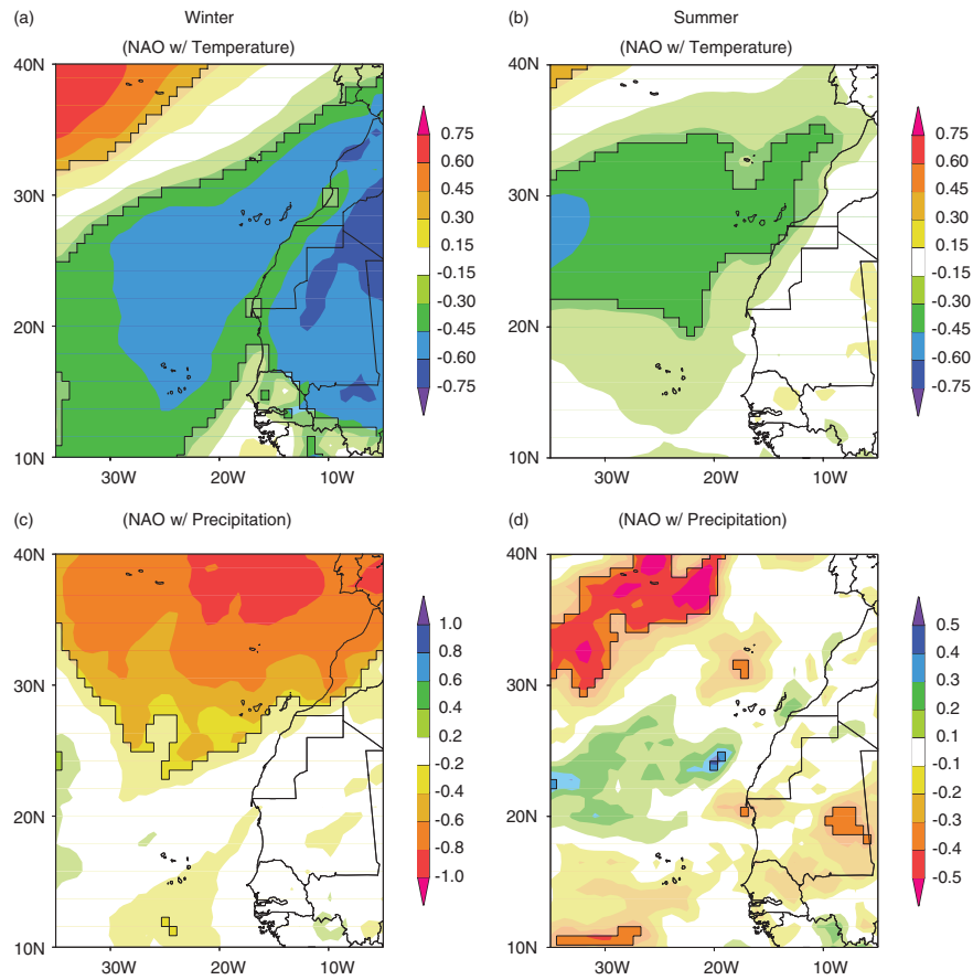
Figure 7. The correlation coefficient between the detrended anomalies of our extended Azores station-based NAOI with 2-m air temperature (a, b) and surface precipitation (c, d) from the ERA-Interim reanalysis across 1979–2011/2012 during winter (DJF) and summer (JJA). Black lines indicate areas statistically significant at 10%.
