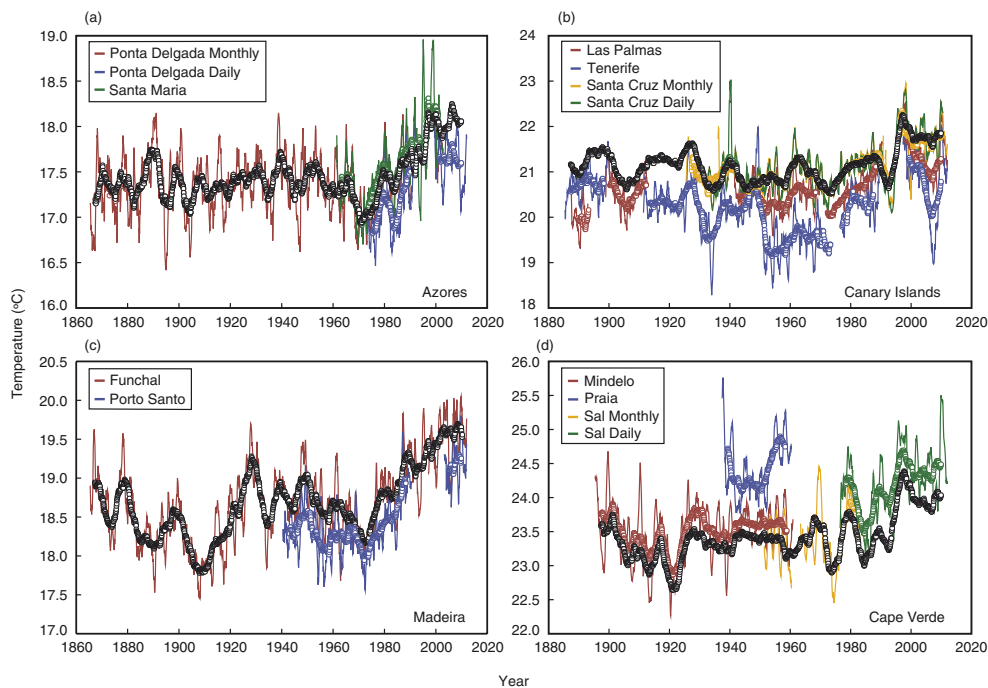
Figure 5. The reconstructed monthly time series of (a) the Azores, (b) the Canary Islands, (c) Madeira and (d) Cape Verde. The 12-month running means of each station used in the reconstruction (as lines) and the 60-month running means of the stations (as circles, black circles indicate the 60-month running mean of the final island time series) are displayed.
