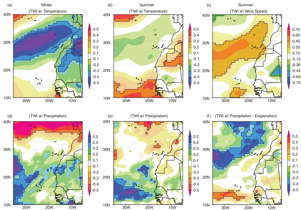
Figure 8. The correlation coefficient between the detrended anomalies of our station-based TWI with 2-m air temperature (a, b), wind speed anomalies (c), surface precipitation (d, e), and P–E (f) from the ERA-Interim reanalysis across 1979–2011/2012 during winter (only for temperature and precipitation) and summer. Black lines indicate areas statistically significant at 10%.
