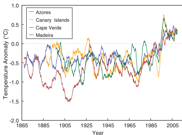
Figure 6. The temperature anomaly (1981–2010 base) for each of the four Macaronesian regions (60-month running mean).
