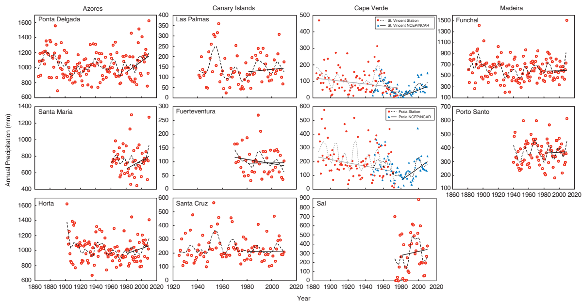
Figure 9. Annual precipitation (mm) records from various Macaronesian sites with their 1981–2010 Thiel-Sen trend line and long-term 11-year LOESS filters.
