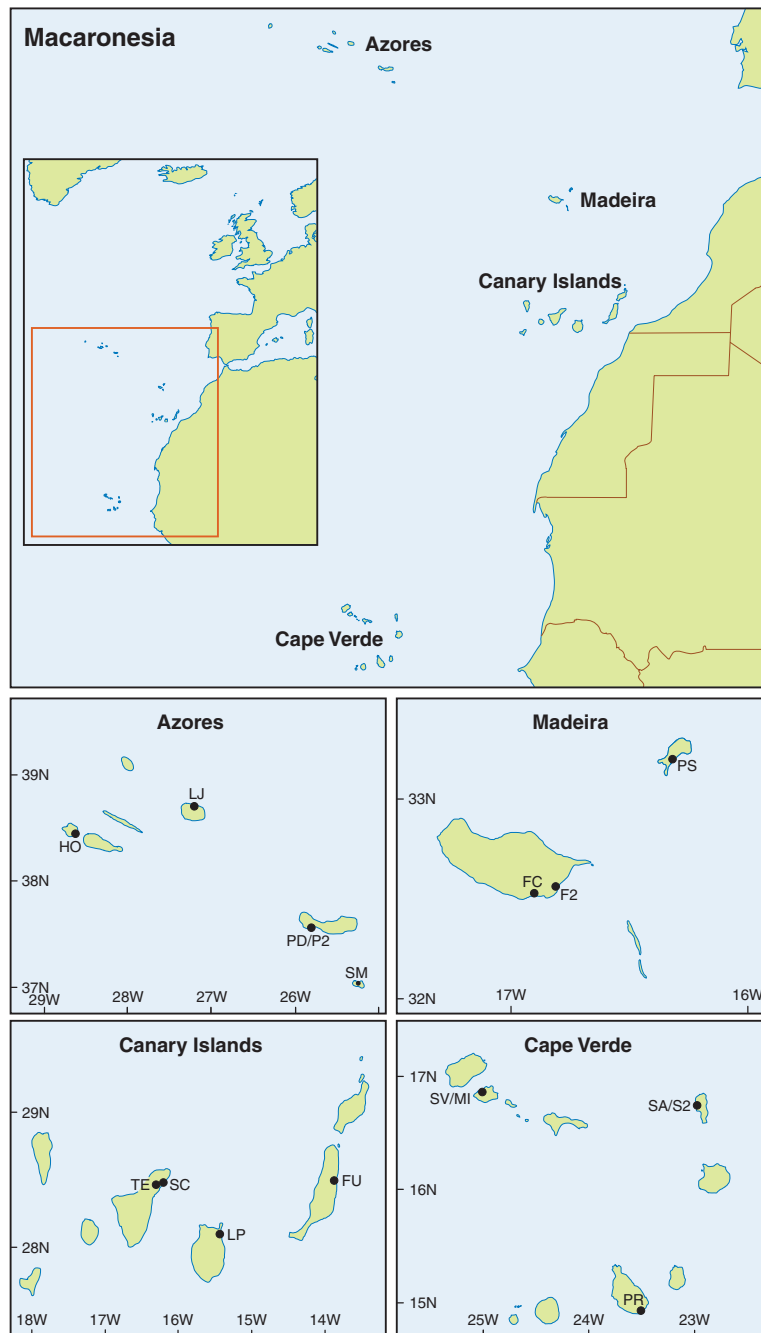
Figure 1. Map of the Macaronesian region illustrating its location within the North Atlantic Ocean. The Azores (top left), Canary Islands (bottom left), Madeira (top right) and Cape Verde (bottom right) island chains are enhanced and marked with the meteorological stations used in this article (Table 1).
