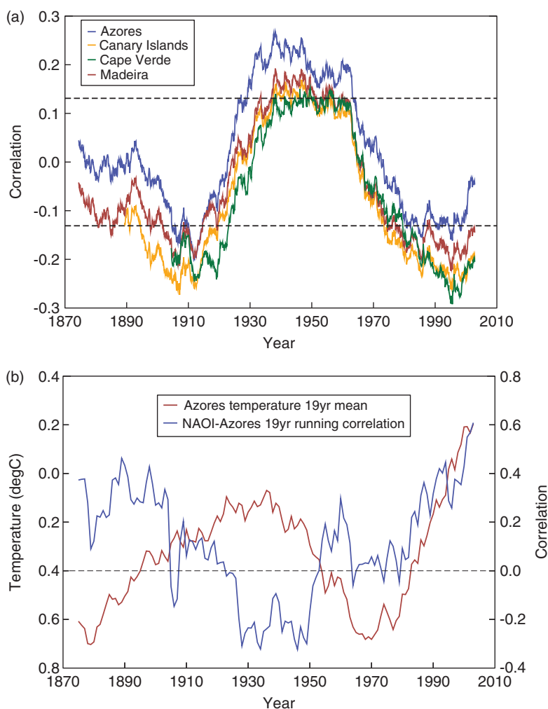
Figure 10. (a) The running correlation (19-year sliding window) between detrended monthly Macaronesian temperature anomalies and the monthly NAOI (dashed lines indicate the boundaries of 95% statistical significance for the correlations) and (b) the running correlation (19-year sliding window) between the detrended Azores winter temperature anomalies and detrended winter NAOI in addition to the 19-year running mean of the Azores winter temperature anomalies.
