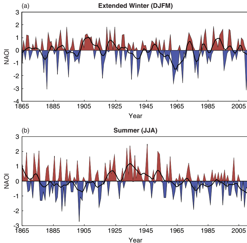
Figure 2. The station-based, (a) extended winter (DJFM) and (b) summer (JJA) North Atlantic Oscillation index 1865–2012. The northern station is a combination of Stykkisholmur/Reykjavik SLP record, and the southern station is our extended Ponta Delgada SLP record. Black lines illustrate an 11-year LOESS filter.
