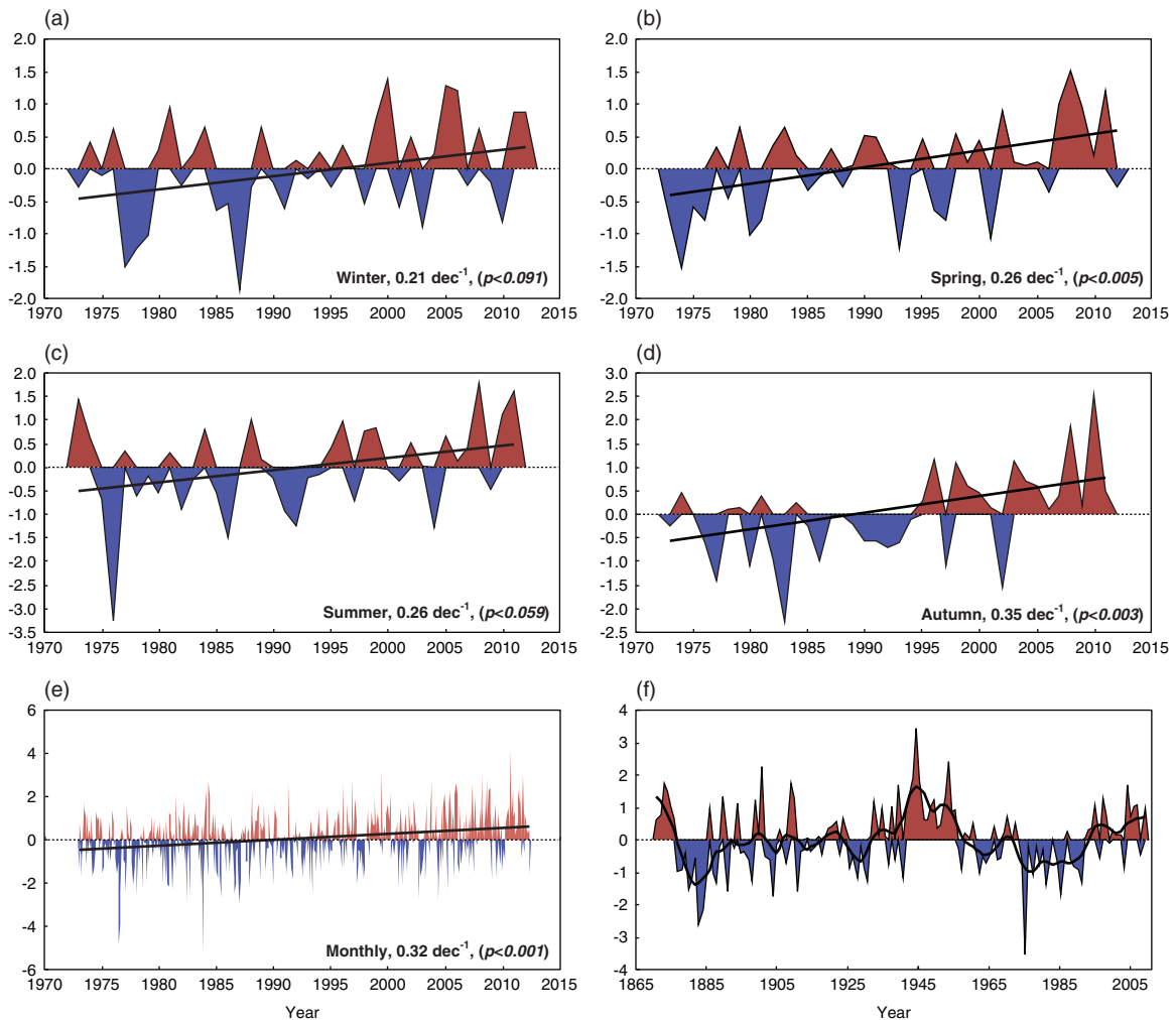
Figure 4. (a) The station-based seasonal (a–d) and monthly (e) Trade Wind index, 1973–2012 and (f) the extended summer (JJA) Trade Wind index, 1871–2010. The northern station is the SLP record from Ponta Delgada, and the southern station is the SLP record from Sal. The black lines (a–e) represent the 1973–2011/2012 Thiel-Sen trends and (f) an 11-year LOESS filter.
