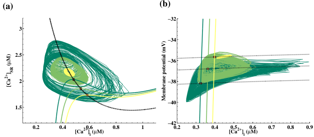
FIGURE 3. Nullcline analysis of the action of varying Ca^{2+} influx via NSSCs. Phase diagram for changes in the parameter A , with (a) membrane potential held constant at -30\text{mV} , and (b) [Ca^{2+}]_{SR} held constant at 1\mu\text{M} . Dark green colour is for A=2.3\mu\text{M s}^{-1} , light green colour for A=2.8\mu\text{M s}^{-1} , and yellow colour for A=3.3\mu\text{M s}^{-1} . x -nullclines ( [Ca^{2+}]_i ) are coloured according to the same pattern. Results are presented for an arbitrary cell within the computational domain, and take into account coupling conditions. Assorted phase plots and equilibria are obtained for different cells, but all present the same generic characteristics.
