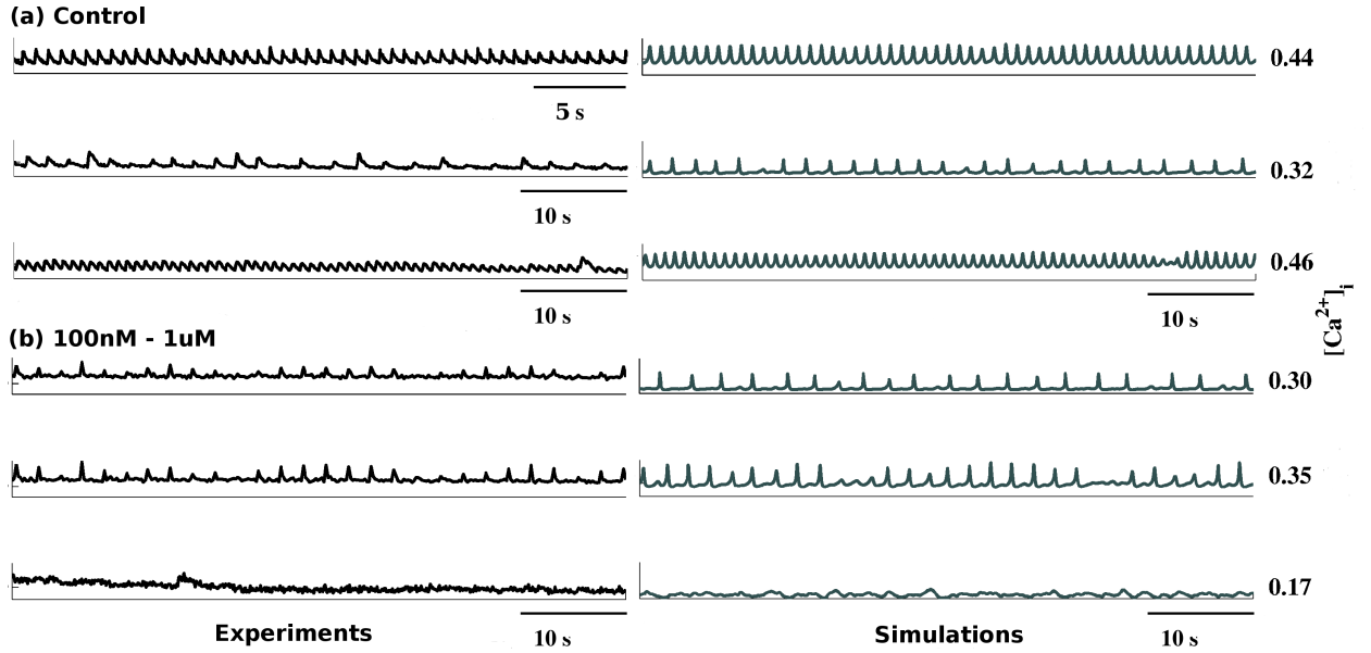
FIGURE 4. Comparison of numerical results and experimental traces for increasing concentrations of verapamil. (a) Control (no drug) and (b) 100\text{nM} - 1\mu\text{M} . For each figure, the left panel corresponds to the time amplitude series of Ca^{2+} fluorescence, obtained from the experiments. The right panel (grey lines) represent the time amplitude series of Ca^{2+} oscillations obtained with the mathematical model. The mean [Ca^{2+}]_i value (in \mu\text{M} ) in each scenario is given on the right hand side of each trace.
