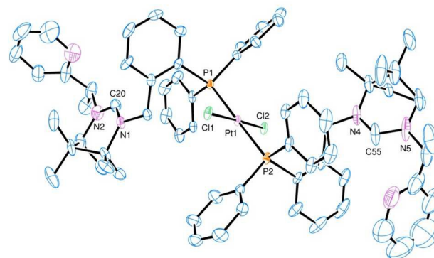
Figure 7. The molecular structure of \text{trans-}[\text{Pt}(\kappa\text{-}P\text{-}N^{\text{Me}}\text{CHP})_2\text{Cl}_2](\text{PF}_6)_2 , 11 . Hydrogen atoms, lattice solvent and \text{PF}_6^- counterions are omitted for clarity. Selected bond lengths (Å) and angles ( ^\circ ): Pt1-P1 2.3068(17); Pt1-P2 2.3102(17); Pt1-C11 2.3026(19); Pt1-Cl2 2.2983(19), P1-Pt1-C11 93.15(7); P1-Pt1-Cl2 86.68(7); P2-Pt1-C11 86.73(7); P2-Pt1-Cl2 93.46(7); P1-Pt1-P2 179.09(17).
