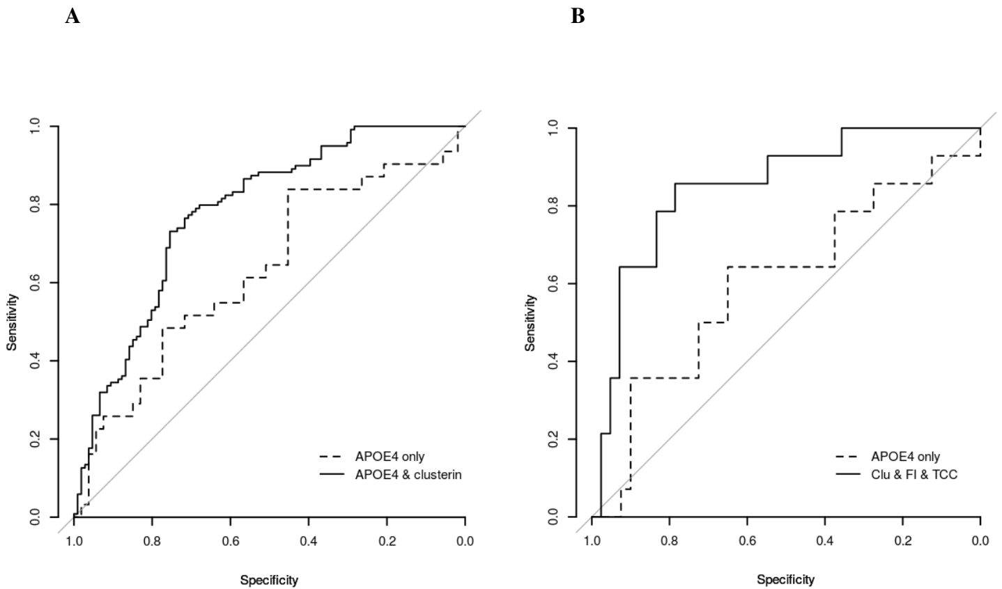
Figure 1. ROC curves.
