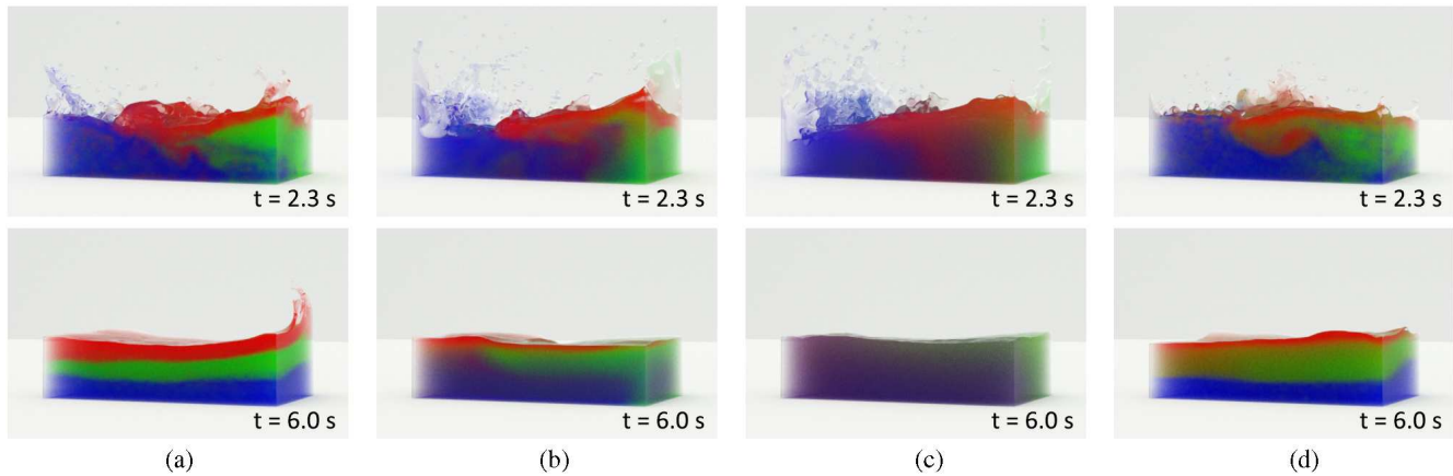
Fig. 3. Three-phase liquid dam breaking (red, green and blue). (a) All three phases are immiscible with each other and they get separated into three layers with clear interfaces. (b) All three phases are miscible with other, and with the diffusion effect disabled they get mixed due to interaction between phases. (c) All three phases are miscible with each other, and with the diffusion effect enabled they get mixed more uniformly. (d) The red and blue phases are miscible with each other, but are both immiscible with the blue phase.
