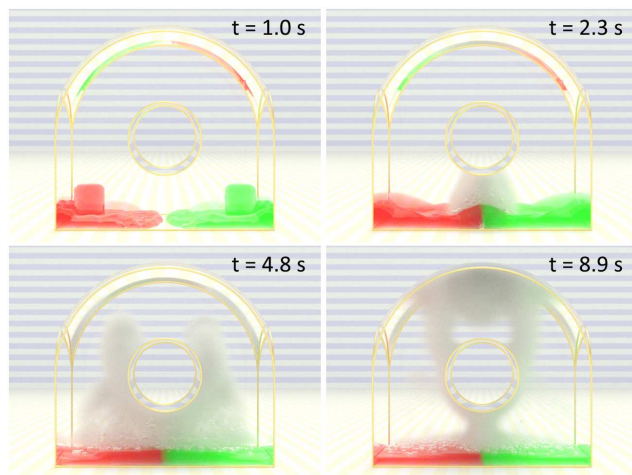
Fig. 7. Vaporization. The dome is filled with transparent air, and from two magic sources red and green liquids are injected into the dome. The two liquids meet at the centre of the floor and react to produce a vapor phase, which rises towards the ceiling. The density ratio is Red liquid:Green liquid:Transparent air:Vapor phase = 1000:1000:2:1.
