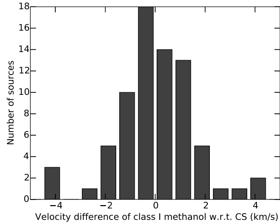
Figure 13. The distribution of velocity offsets between the peak velocity of class I \text{CH}_3\text{OH} and CS (1–0). The bin size was chosen to be 0.75 \text{ km s}^{-1} . The histogram is approximated by a Gaussian with a mean velocity 0 \pm 0.2 \text{ km s}^{-1} and standard deviation 1.5 \pm 0.1 \text{ km s}^{-1} .
