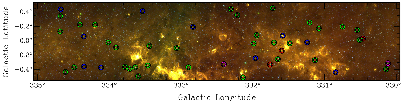
Figure 8: Spitzer GLIMPSE 3-colour (RGB = 3.6, 5.8 and 8.0\,\mu\text{m} ) image with MALT-45 positions of detected \text{SiO} (1–0) v = 1, 2, 3 masers (circle symbols). The circles have been colour-coded by the vibrational modes within each region. Red: region containing v = 1, 2, 3 maser emission; green: v = 1, 2 ; blue: v = 1 ; magenta: v = 2 .
