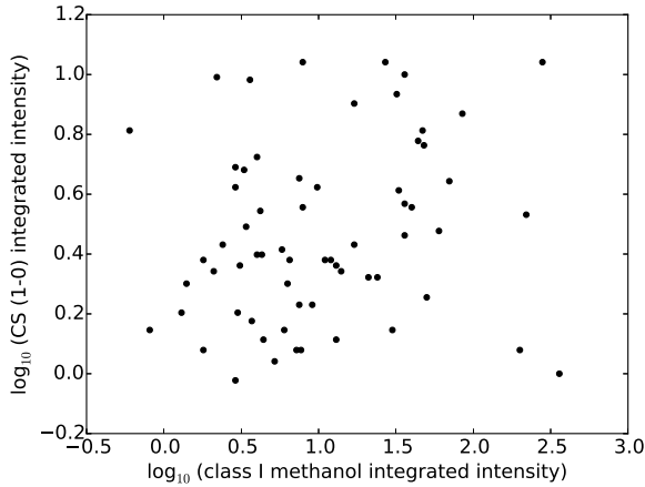
Figure 12. A log-log scatter plot of class I \text{CH}_3\text{OH} and CS integrated intensities. Units of integrated intensity are \text{Jy km s}^{-1} for class I \text{CH}_3\text{OH} , and \text{K km s}^{-1} for CS. There is no significant correlation observed in either subpopulation, or the total population.
