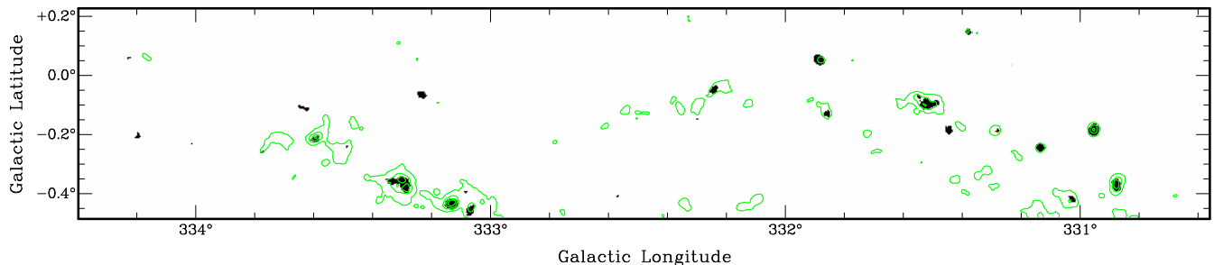
Figure 7: Auto-correlated map of \text{SiO} (1–0) v = 0 , overlaid with \text{CS} (1–0) thermal emission contours. This image shows \text{SiO} emission at and above 0.04\,\text{K} ( \sim 1.5\sigma ). Contour levels are 14, 34, ...74 per cent of 2.62\,\text{K} .
