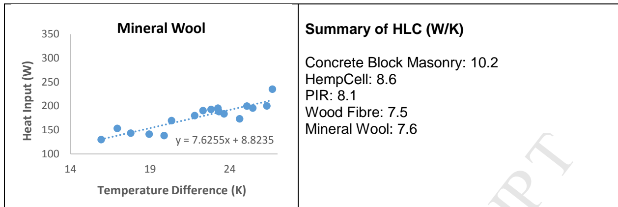
Fig. 12. Coheating regression plot using Method 2.
