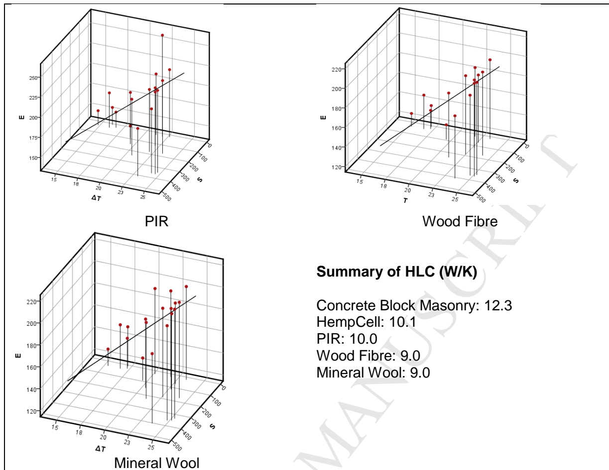
Fig. 14. Coheating regression plot using Method 4.
