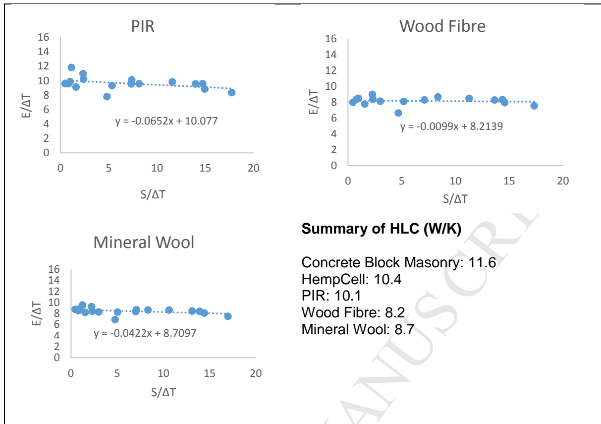
Fig. 13. Coheating regression plot using Method 3.
