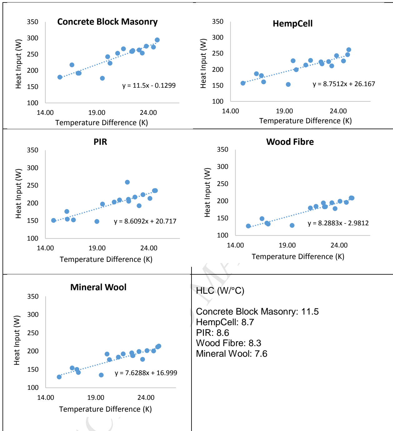
Fig. 11. Coheating regression plot using Method 1.
