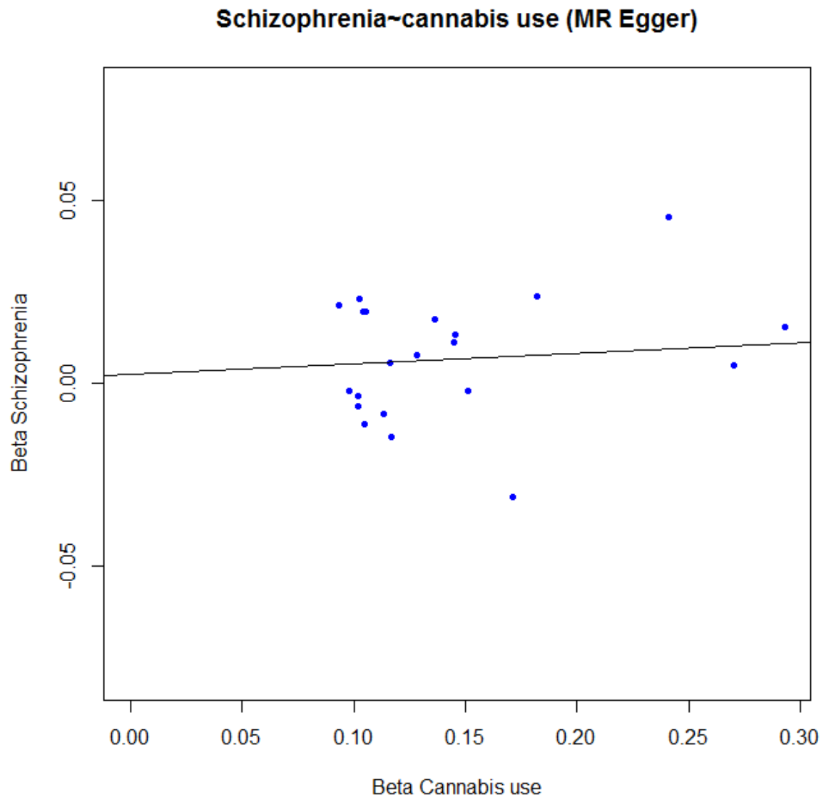
Supplementary figure 1: MR Egger regression of cannabis initiation predicting risk of schizophrenia.
