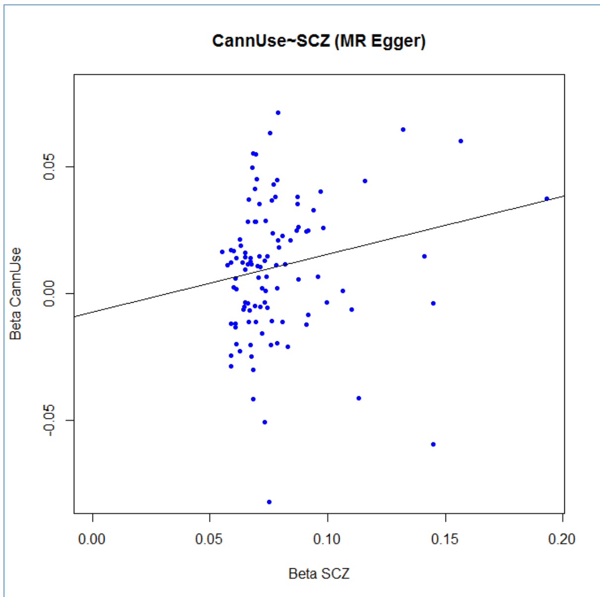
Supplementary Figure 2: MR Egger regression risk of schizophrenia predicting cannabis initiation.
