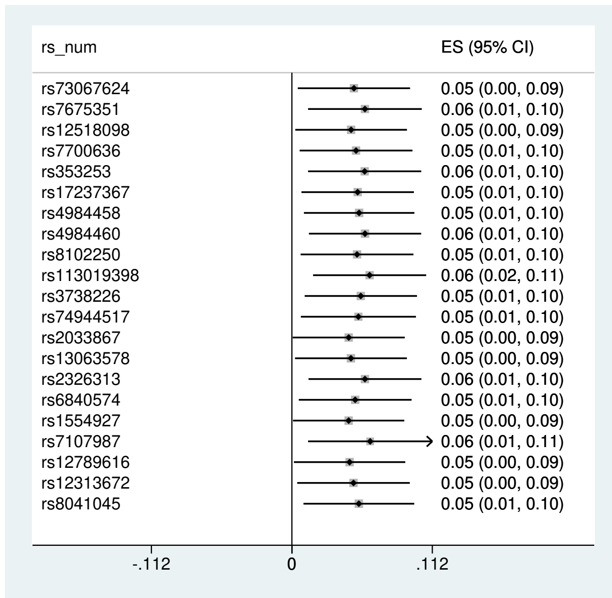
Supplementary Figure 3: Forest plot showing the effect size and confidence intervals of Mendelian randomization associations between cannabis initiation and risk of schizophrenia, systematically removing each cannabis initiation SNP in turn
