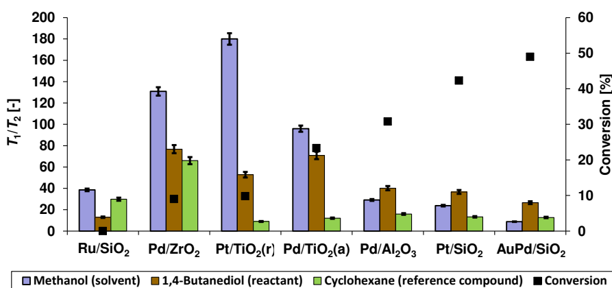
Figure 34. Conversion and T_1/T_2 ratio values of methanol (solvent), 1,4-butanediol (reactant) and cyclohexane (reference compound) in different catalysts. The relative error in the T_1/T_2 ratio is approximately 3%. The T_1/T_2 value for each of the bulk liquids (methanol, 1,4-butanediol and cyclohexane) is equal to one.
