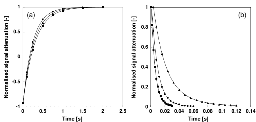
Figure 23. (a) T_1 inversion recovery and (b) T_2 CPMG relaxation data of 1,4-butanediol in different catalysts: (■) Pd/ZrO 2 ; (●) AuPd/SiO 2 ; (▲) Ru/SiO 2 . The values of the relaxation times are: T_1 = 301 ms and T_2 = 6 ms for Pd/ZrO 2 ; T_1 = 242 ms and T_2 = 9 ms for AuPd/SiO 2 ; T_1 = 272 ms and T_2 = 21 ms for Ru/SiO 2 . The solid lines are fits to the data using the theoretical expressions to (a) inversion recovery 24 and (b) CPMG decay. 24
