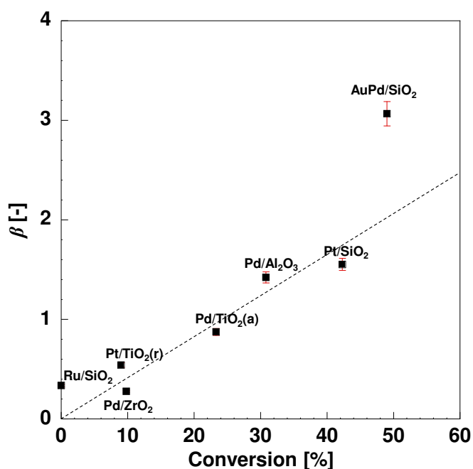
Figure 45. Plot of \beta , as defined in Equation (2) against catalytic conversion. Note that (a) indicates TiO 2 anatase and (r) indicates TiO 2 rutile. The dotted line is a guide to the eye.
