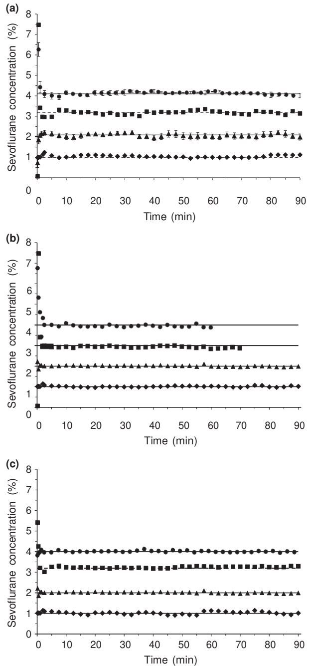
Figure 3 Sevoflurane output concentrations of the anaesthetic delivery device at various stirring rates with an input flow of 1 \text{ l.min}^{-1} nitrogen at 20^\circ\text{C} .
