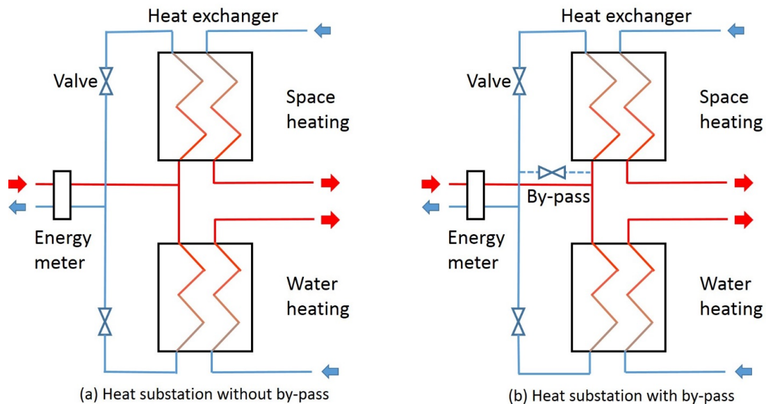
Fig. 8 simplified substation
