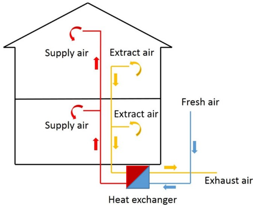
Fig. 10 Building heat recovery
