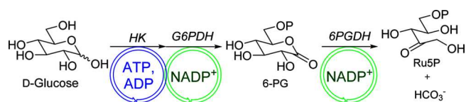
Figure 4. Conversion of D-glucose to ribulose 5-phosphate (Ru5P) by hexokinase (HK), glucose 6-phosphate dehydrogenase (G6PDH), and 6-phosphogluconate dehydrogenase (6-PGDH). Details of the ATP and NADP + recycling systems are described in Figure 3 and in the text.
