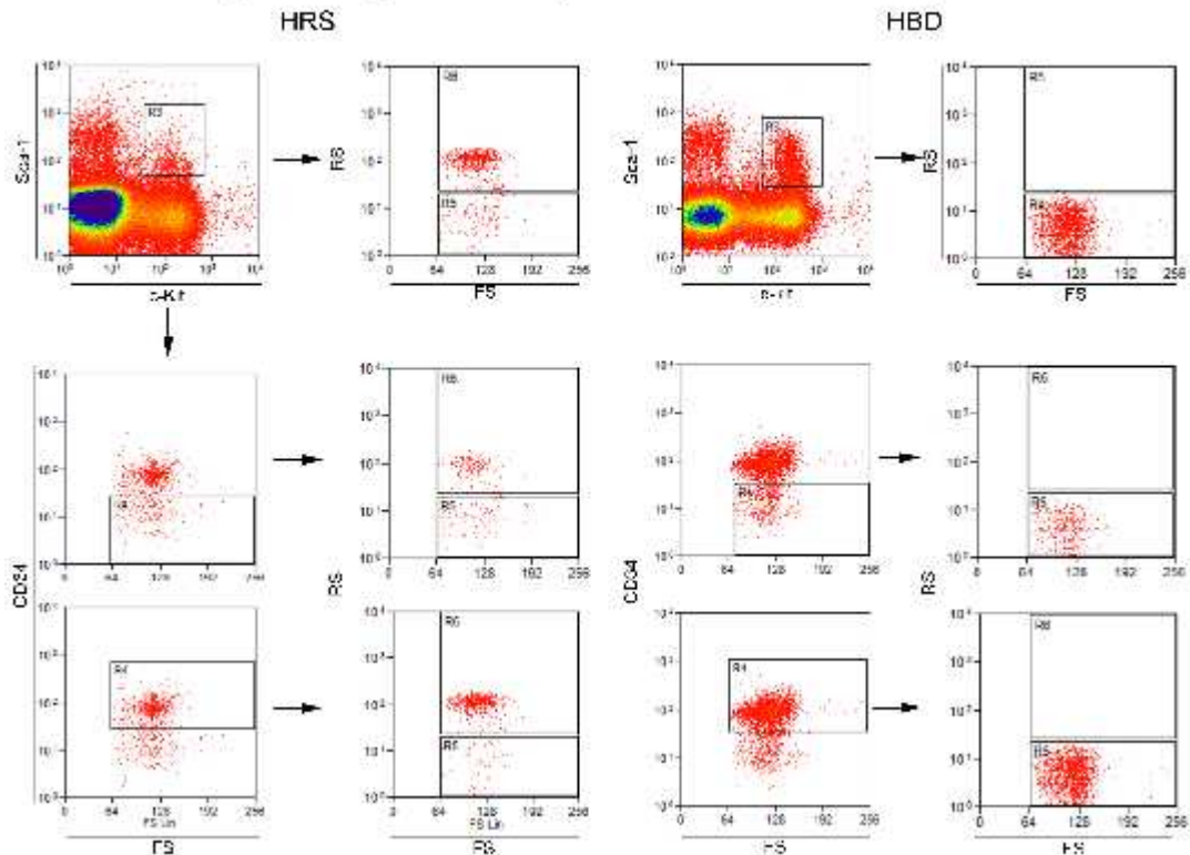
Figure 6. Analysis of Hhex Expression in the Adult HSC Compartment
