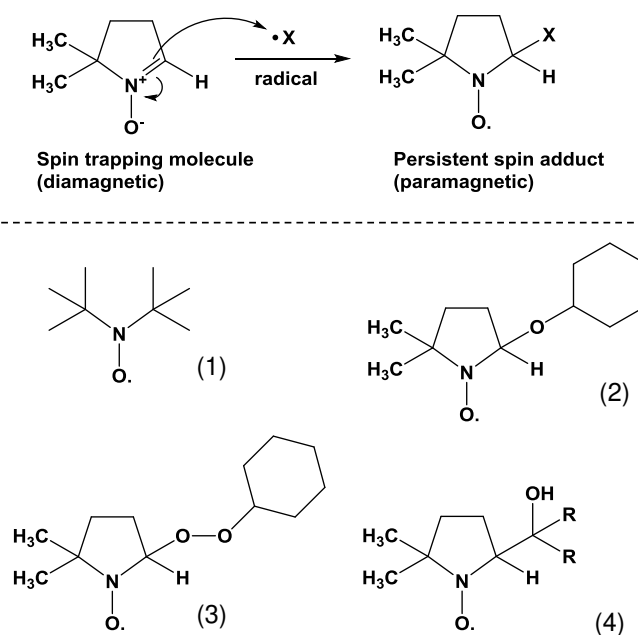
Figure 5. (A) Principle of the spin trapping methodology: fast selective addition (trapping) of short-lived radicals to a diamagnetic spin trap, usually a nitrone or a nitroso compound, such as 5,5-dimethyl-1-pyrroline-N-oxide (DMPO). The product of this addition (spin adduct) is a persistent free radical (nitroxide) with sufficiently long lifetime to enable detection by conventional EPR spectroscopy. (B) Proposed structures of the DMPO spin-adducts detected in the CHHP decomposition in cyclohexane by AgPd/MgO catalyst prepared by sol-immobilization (cross reference with Figure 4): (1) di- tert -butyl-nitroxide derivative, (2) DMPO-O-C 6 H 11 spin adduct, (3) DMPO-O 2 -C 6 H 11 adduct, and (4) carbon centred adduct, which is possibly a DMPO-C(OH)R 2 species.
