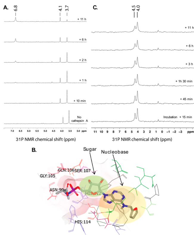
Figure 4. Metabolism and serum stability of KR ProTides. (A) ^{31}\text{P} NMR of cathepsin A mediated in vitro degradation of KR ProTide 14 . (B) Docking of metabolite 17 into the crystal structure of Hint-1 to predict the cleavage of the P–N bond. (C) Stability of KR ProTide 14 in human serum over 12 h as monitored by ^{31}\text{P} NMR.
