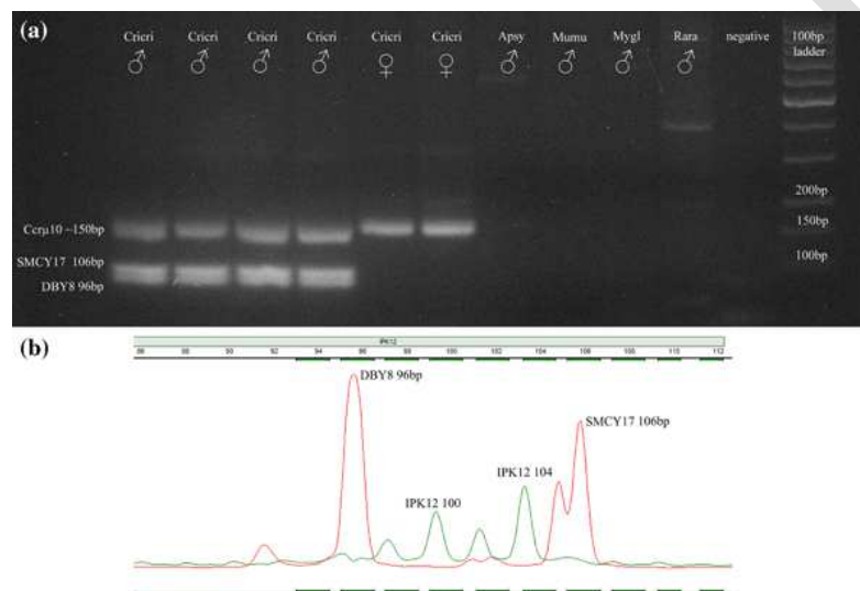
Figure 1: a Electrophoresis of the simple multiplex PCR products of SMCY17-Cricri and DBY8-Cricri, and the microsatellite Ccri10 as positive control. Tissue extracts of male and female common hamsters ( Cricri ) and four male non-target rodent species ( Apsy = Apodemus flavicollis , Mimu = Mus musculus , Mygl = Myodes glareolus , Rara = Rattus norvegicus ). b Electropherogram of the complex multiplex for a male hamster showing SMCY17-Cricri, DBY8-Cricri and microsatellite IPK12 peaks.
