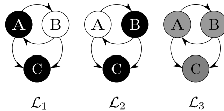
Figure 6: The skeptical operator is not strategy-proof.
